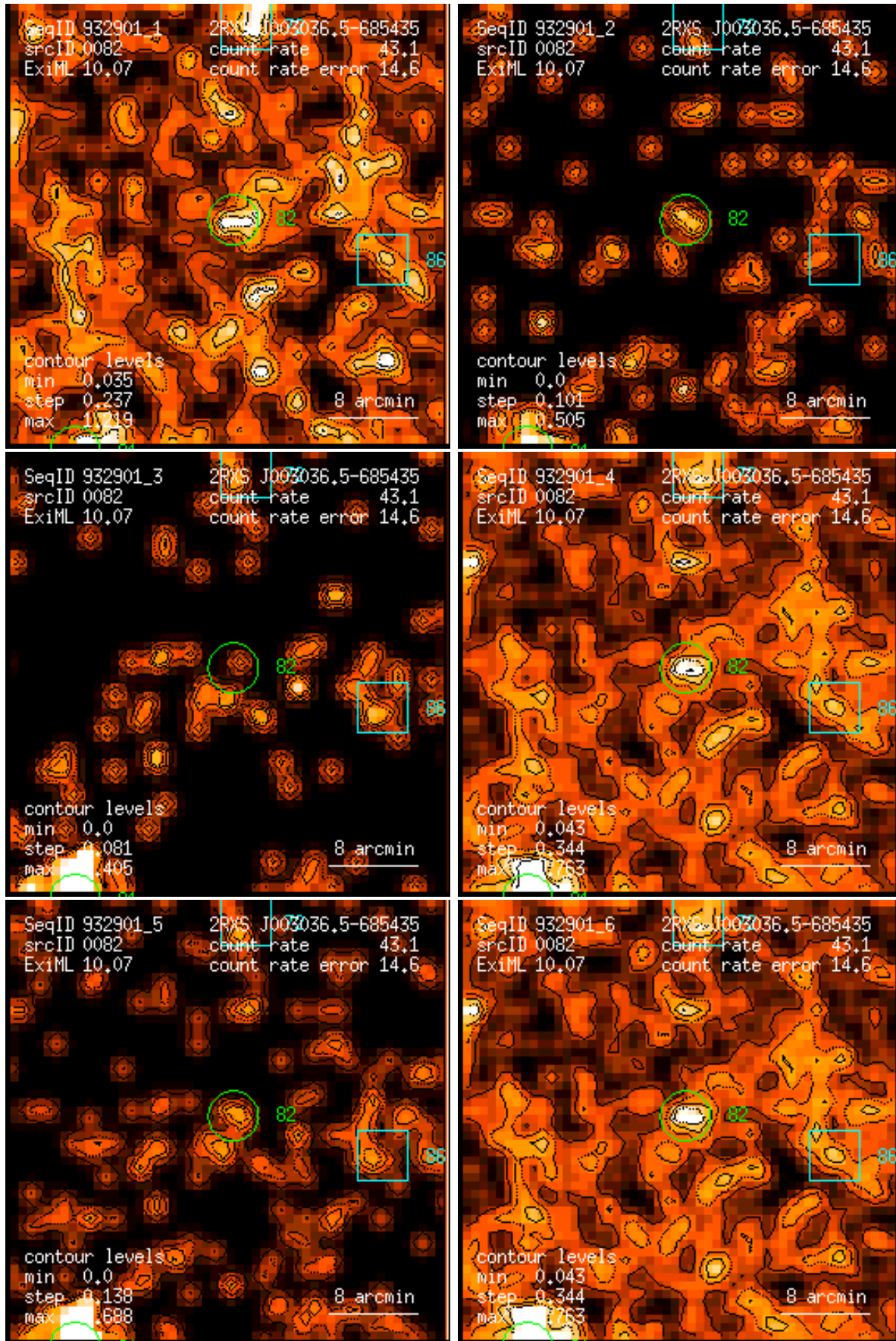
Figure 82: RASS 932901: detection 0082: band rate images, Gaussian filter: (1) PSPC channels 11 – 41, (2) 52 – 90, (3) 91 – 201, (4) 11 – 235, (5) 52 – 201, (6) 11 – 201. Broad band rates in counts/ks. Band rate contour levels in counts/ks/arcmin 2 .
