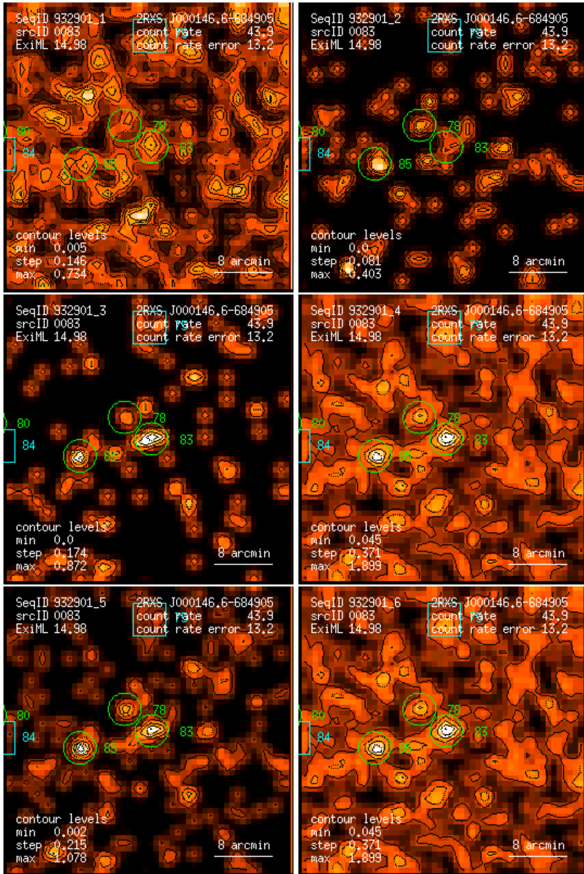
Figure 83: RASS 932901: detection 0083: band rate images, Gaussian filter: (1) PSPC channels 11 – 41, (2) 52 – 90, (3) 91 – 201, (4) 11 – 235, (5) 52 – 201, (6) 11 – 201. Broad band rates in counts/ks. Band rate contour levels in counts/ks/arcmin 2 .
