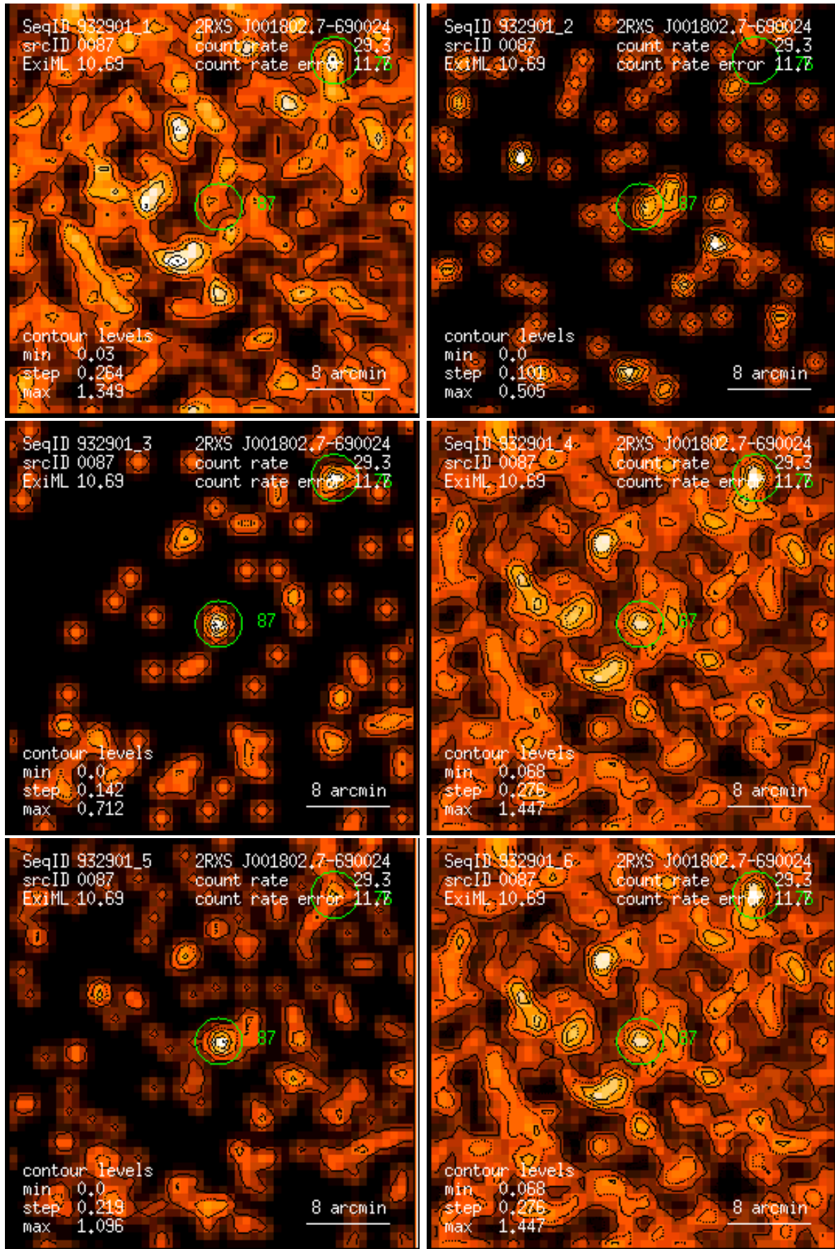
Figure 87: RASS 932901: detection 0087: band rate images, Gaussian filter: (1) PSPP channels 11 – 41, (2) 52 – 90, (3) 91 – 201, (4) 11 – 235, (5) 52 – 201, (6) 11 – 201. Broad band rates in counts/ks. Band rate contour levels in counts/ks/arcmin 2 .
