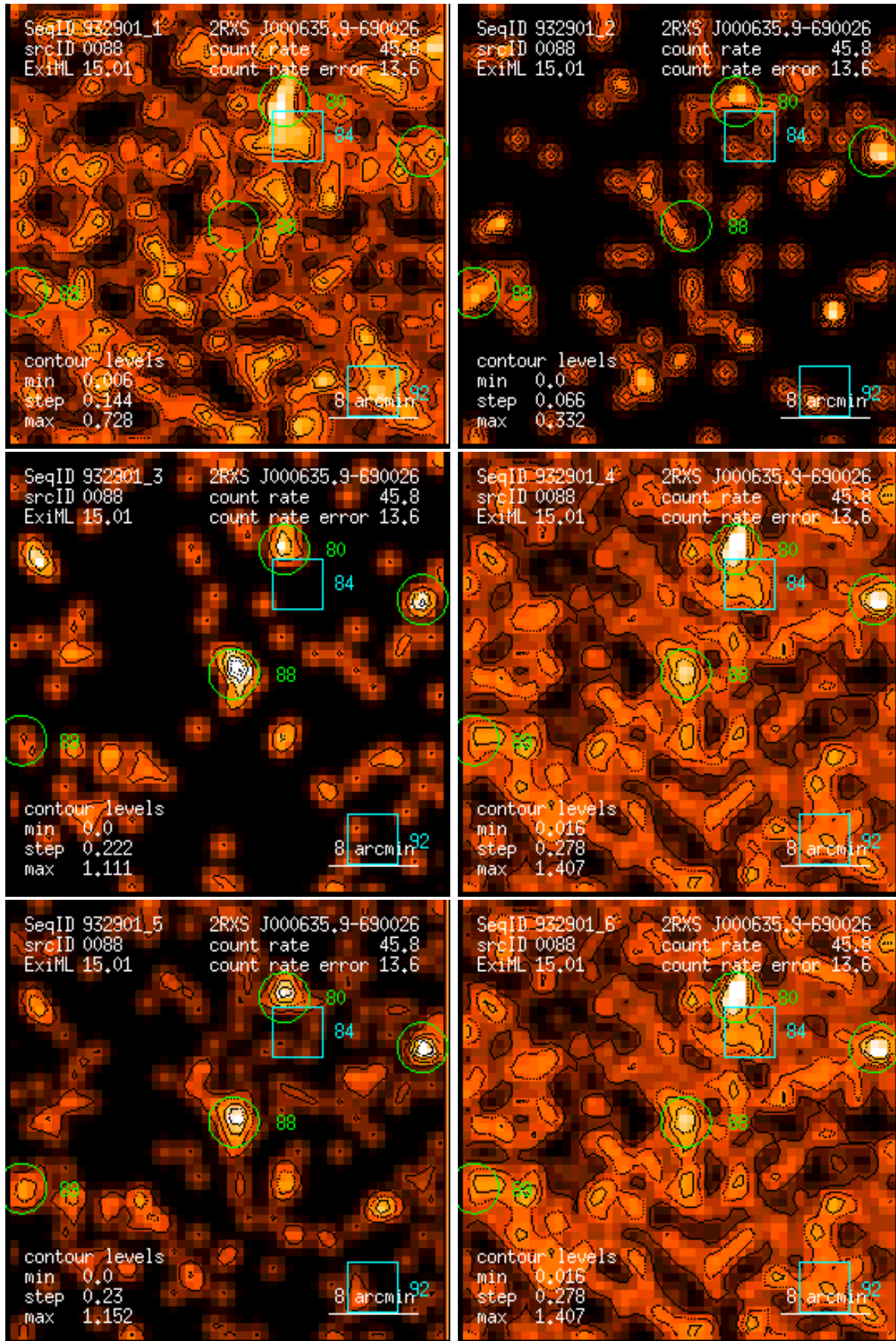
Figure 88: RASS 932901: detection 0088: band rate images, Gaussian filter: (1) PSPC channels 11 – 41, (2) 52 – 90, (3) 91 – 201, (4) 11 – 235, (5) 52 – 201, (6) 11 – 201. Broad band rates in counts/ks. Band rate contour levels in counts/ks/arcmin 2 .
