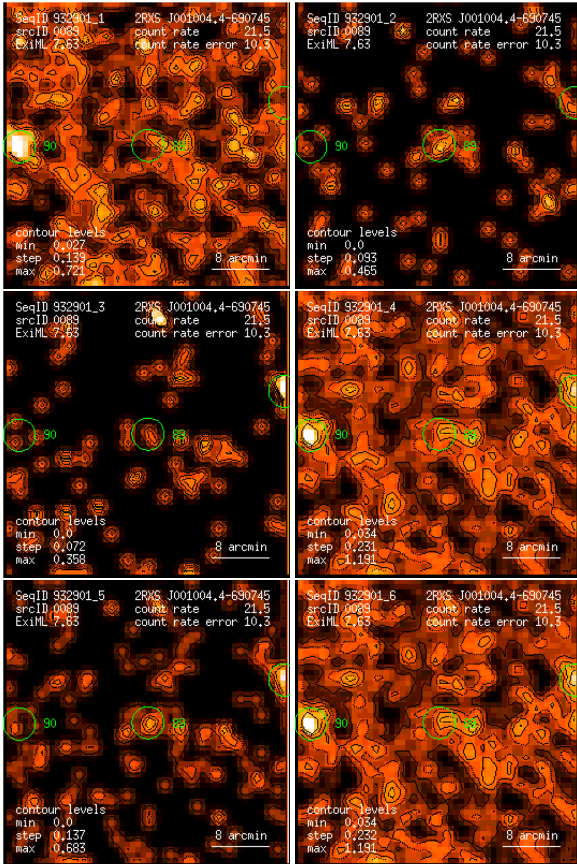
Figure 89: RASS 932901: detection 0089: band rate images, Gaussian filter: (1) PSPC channels 11 – 41, (2) 52 – 90, (3) 91 – 201, (4) 11 – 235, (5) 52 – 201, (6) 11 – 201. Broad band rates in counts/ks. Band rate contour levels in counts/ks/arcmin 2 .
