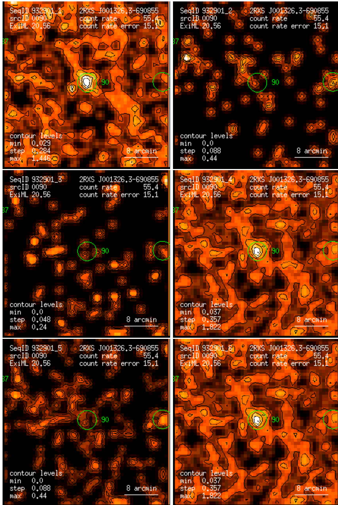
Figure 90: RASS 932901: detection 0090: band rate images, Gaussian filter: (1) PSPC channels 11 – 41, (2) 52 – 90, (3) 91 – 201, (4) 11 – 235, (5) 52 – 201, (6) 11 – 201. Broad band rates in counts/ks. Band rate contour levels in counts/ks/arcmin 2 .
