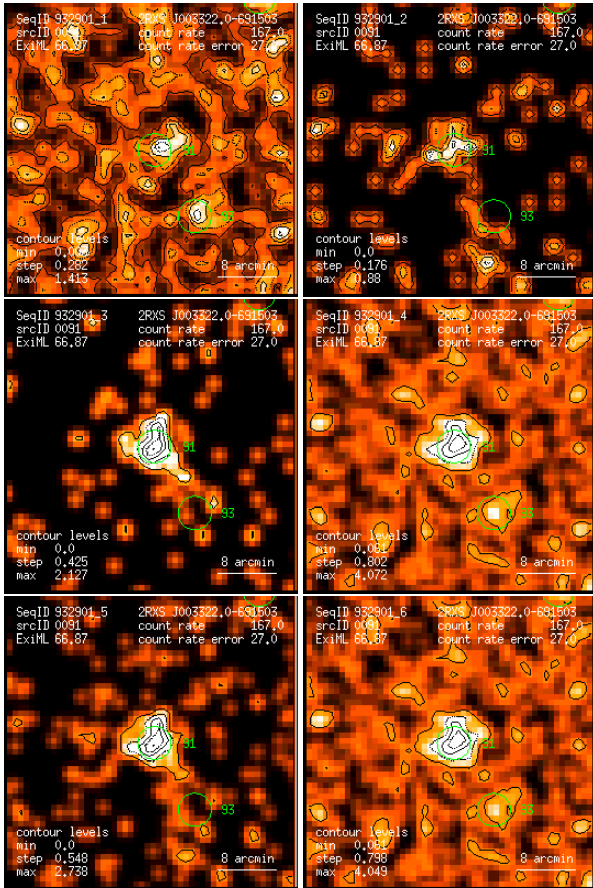
Figure 91: RASS 932901: detection 0091: band rate images, Gaussian filter: (1) PSPC channels 11 – 41, (2) 52 – 90, (3) 91 – 201, (4) 11 – 235, (5) 52 – 201, (6) 11 – 201. Broad band rates in counts/ks. Band rate contour levels in counts/ks/arcmin 2 .
