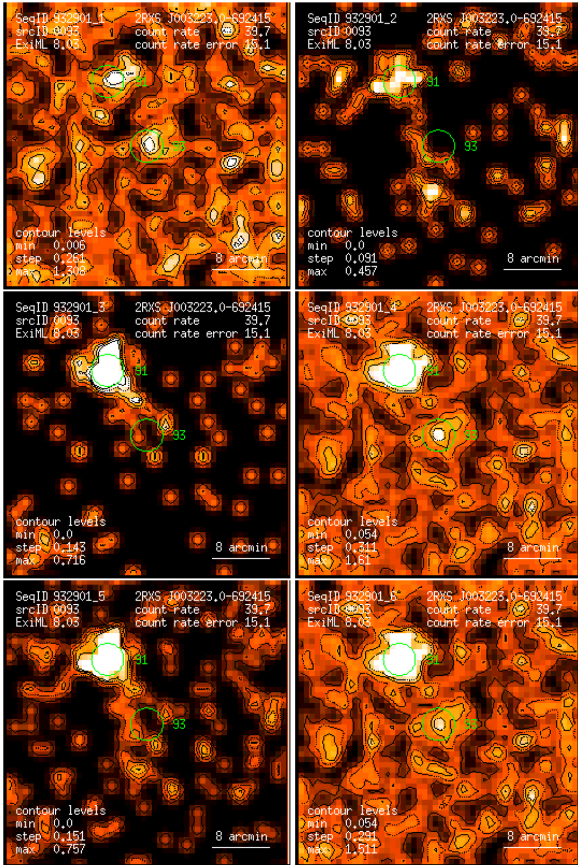
Figure 93: RASS 932901: detection 0093: band rate images, Gaussian filter: (1) PSPC channels 11 – 41, (2) 52 – 90, (3) 91 – 201, (4) 11 – 235, (5) 52 – 201, (6) 11 – 201. Broad band rates in counts/ks. Band rate contour levels in counts/ks/arcmin 2 .
