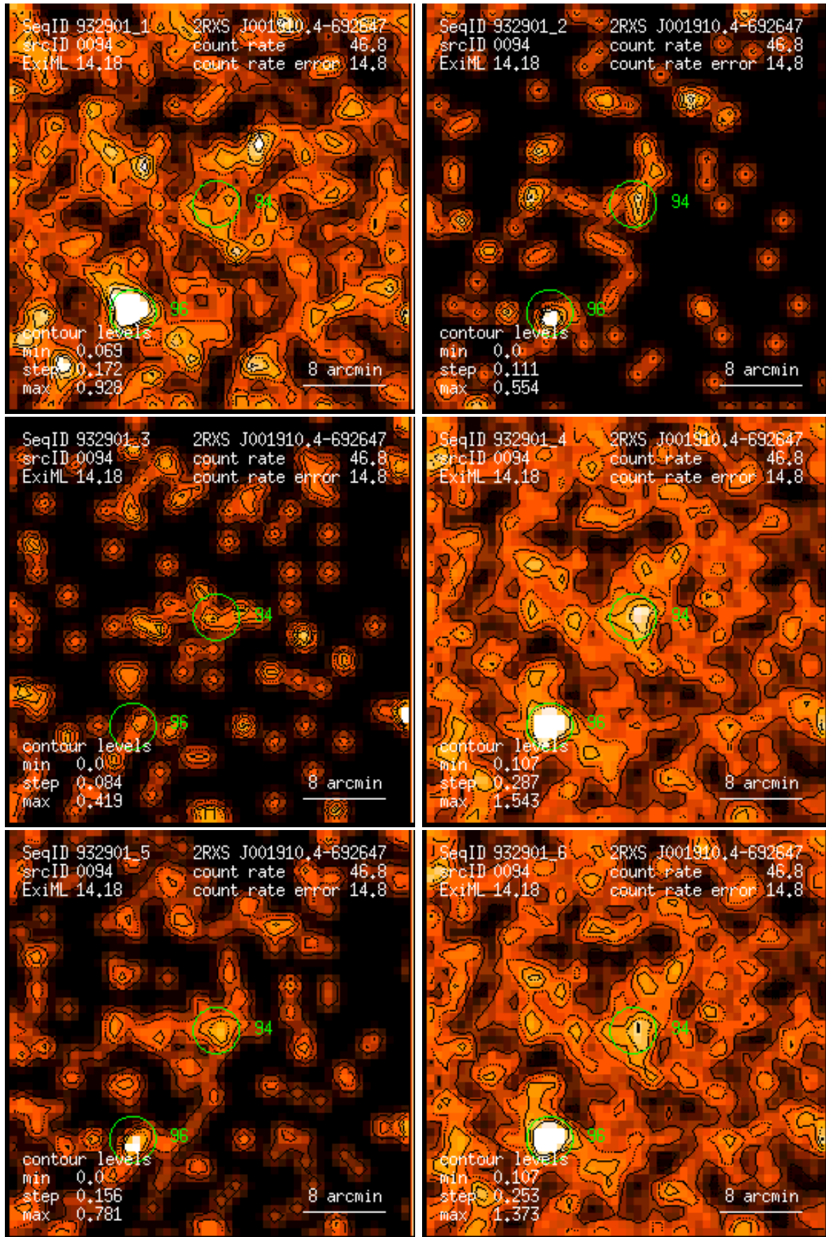
Figure 94: RASS 932901: detection 0094: band rate images, Gaussian filter: (1) PSPC channels 11 – 41, (2) 52 – 90, (3) 91 – 201, (4) 11 – 235, (5) 52 – 201, (6) 11 – 201. Broad band rates in counts/ks. Band rate contour levels in counts/ks/arcmin 2 .
