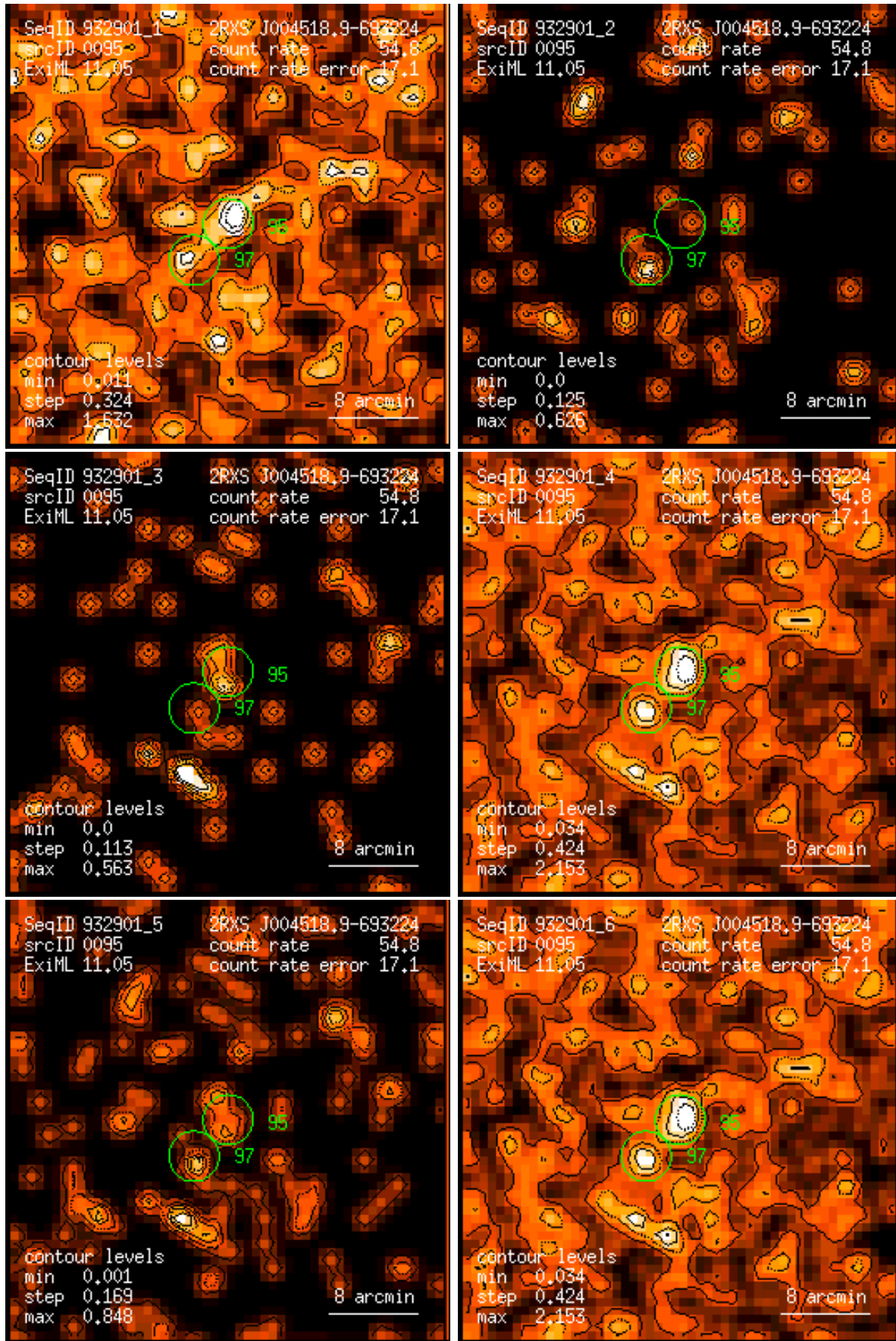
Figure 95: RASS 932901: detection 0095: band rate images, Gaussian filter: (1) PSPC channels 11 – 41, (2) 52 – 90, (3) 91 – 201, (4) 11 – 235, (5) 52 – 201, (6) 11 – 201. Broad band rates in counts/ks. Band rate contour levels in counts/ks/arcmin 2 .
