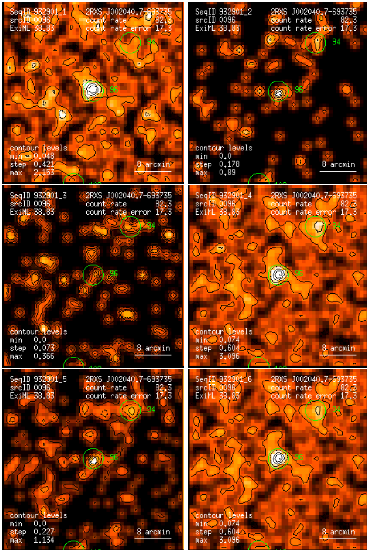
Figure 96: RASS 932901: detection 0096: band rate images, Gaussian filter: (1) PSPC channels 11 – 41, (2) 52 – 90, (3) 91 – 201, (4) 11 – 235, (5) 52 – 201, (6) 11 – 201. Broad band rates in counts/ks. Band rate contour levels in counts/ks/arcmin 2 .
