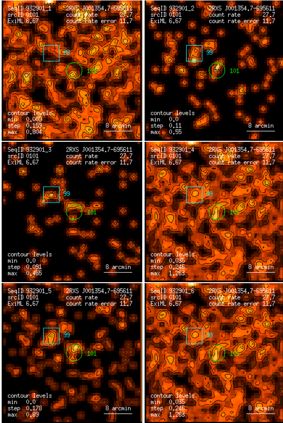
Figure 101: RASS 932901: detection 0101: band rate images, Gaussian filter: (1) PSPC channels 11 – 41, (2) 52 – 90, (3) 91 – 201, (4) 11 – 235, (5) 52 – 201, (6) 11 – 201. Broad band rates in counts/ks. Band rate contour levels in counts/ks/arcmin 2 .
