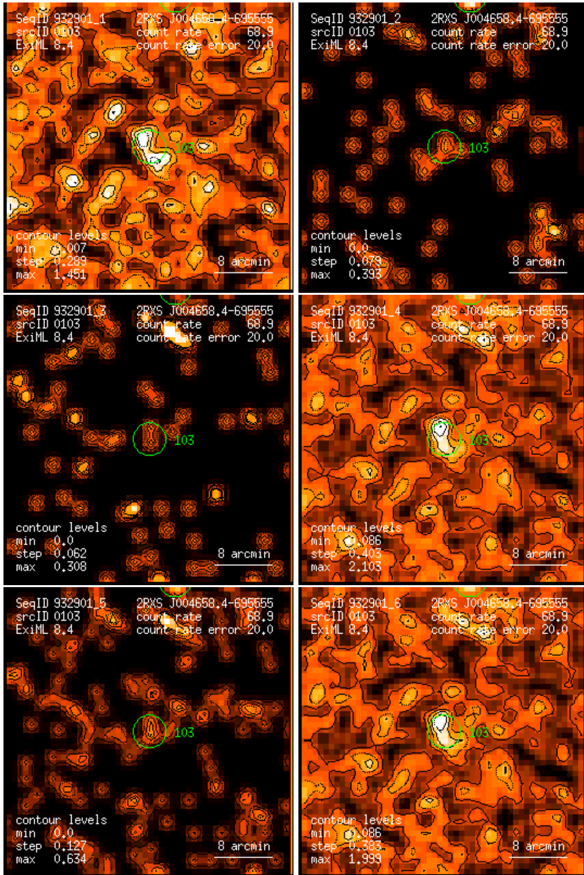
Figure 103: RASS 932901: detection 0103: band rate images, Gaussian filter: (1) PSPC channels 11 – 41, (2) 52 – 90, (3) 91 – 201, (4) 11 – 235, (5) 52 – 201, (6) 11 – 201. Broad band rates in counts/ks. Band rate contour levels in counts/ks/arcmin 2 .
