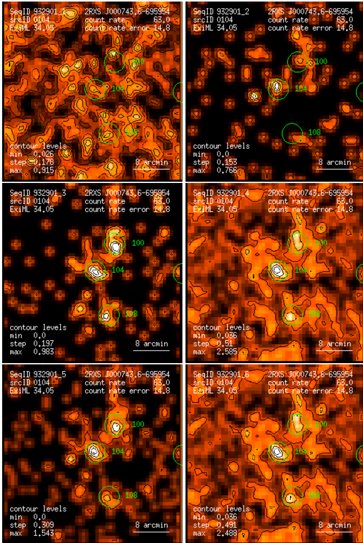
Figure 104: RASS 932901: detection 0104: band rate images, Gaussian filter: (1) PSPC channels 11 – 41, (2) 52 – 90, (3) 91 – 201, (4) 11 – 235, (5) 52 – 201, (6) 11 – 201. Broad band rates in counts/ks. Band rate contour levels in counts/ks/arcmin 2 .
