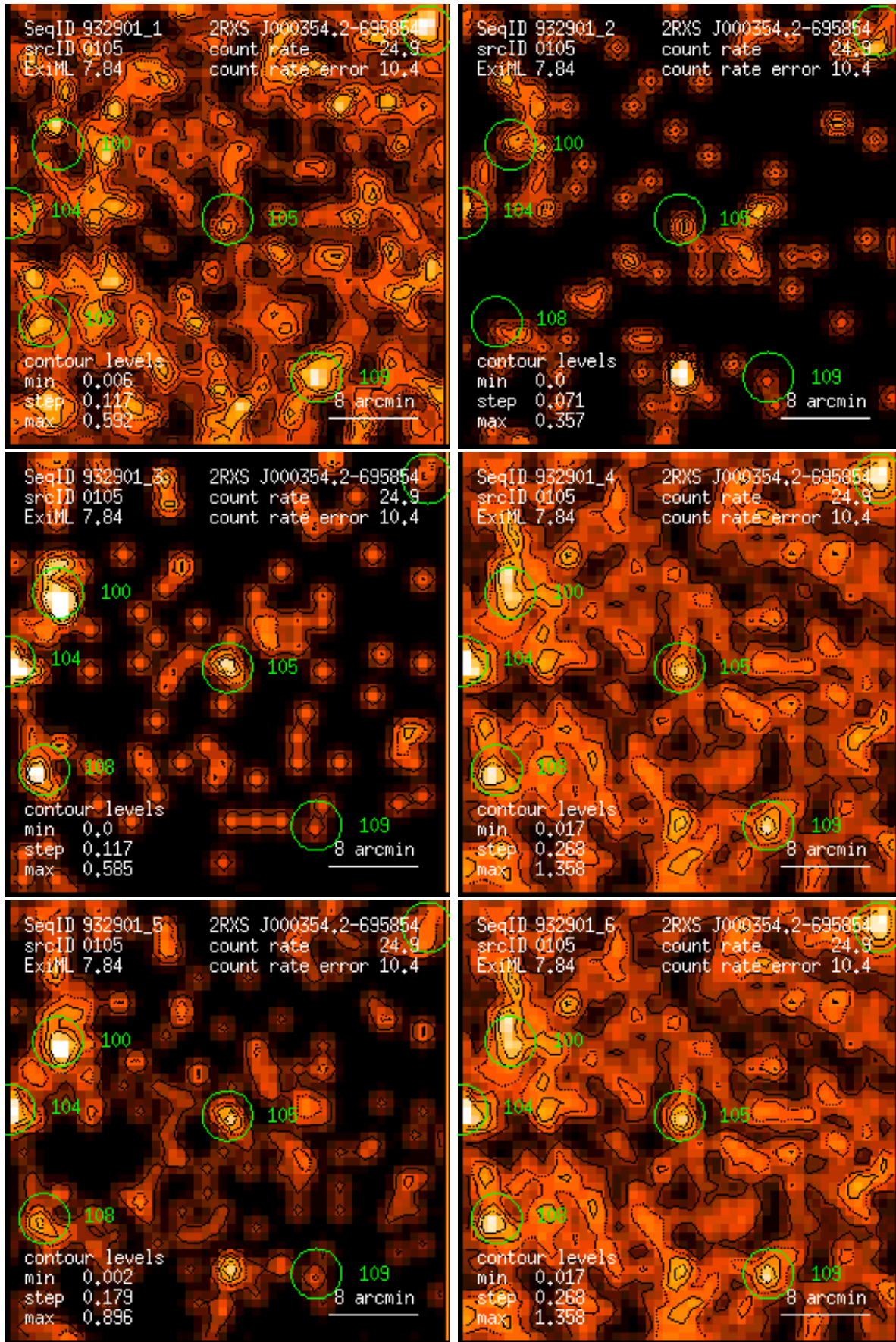
Figure 105: RASS 932901: detection 0105: band rate images, Gaussian filter: (1) PSPC channels 11 – 41, (2) 52 – 90, (3) 91 – 201, (4) 11 – 235, (5) 52 – 201, (6) 11 – 201. Broad band rates in counts/ks. Band rate contour levels in counts/ks/arcmin 2 .
