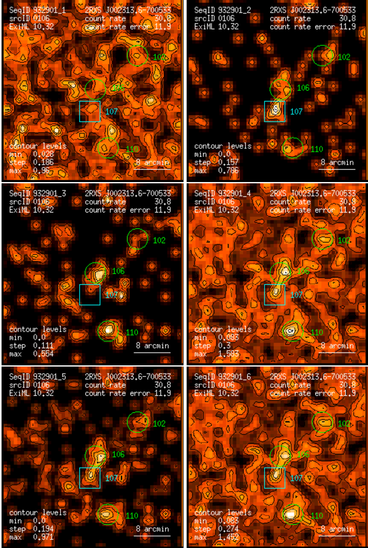
Figure 106: RASS 932901: detection 0106: band rate images, Gaussian filter: (1) PSPC channels 11 – 41, (2) 52 – 90, (3) 91 – 201, (4) 11 – 235, (5) 52 – 201, (6) 11 – 201. Broad band rates in counts/ks. Band rate contour levels in counts/ks/arcmin 2 .
