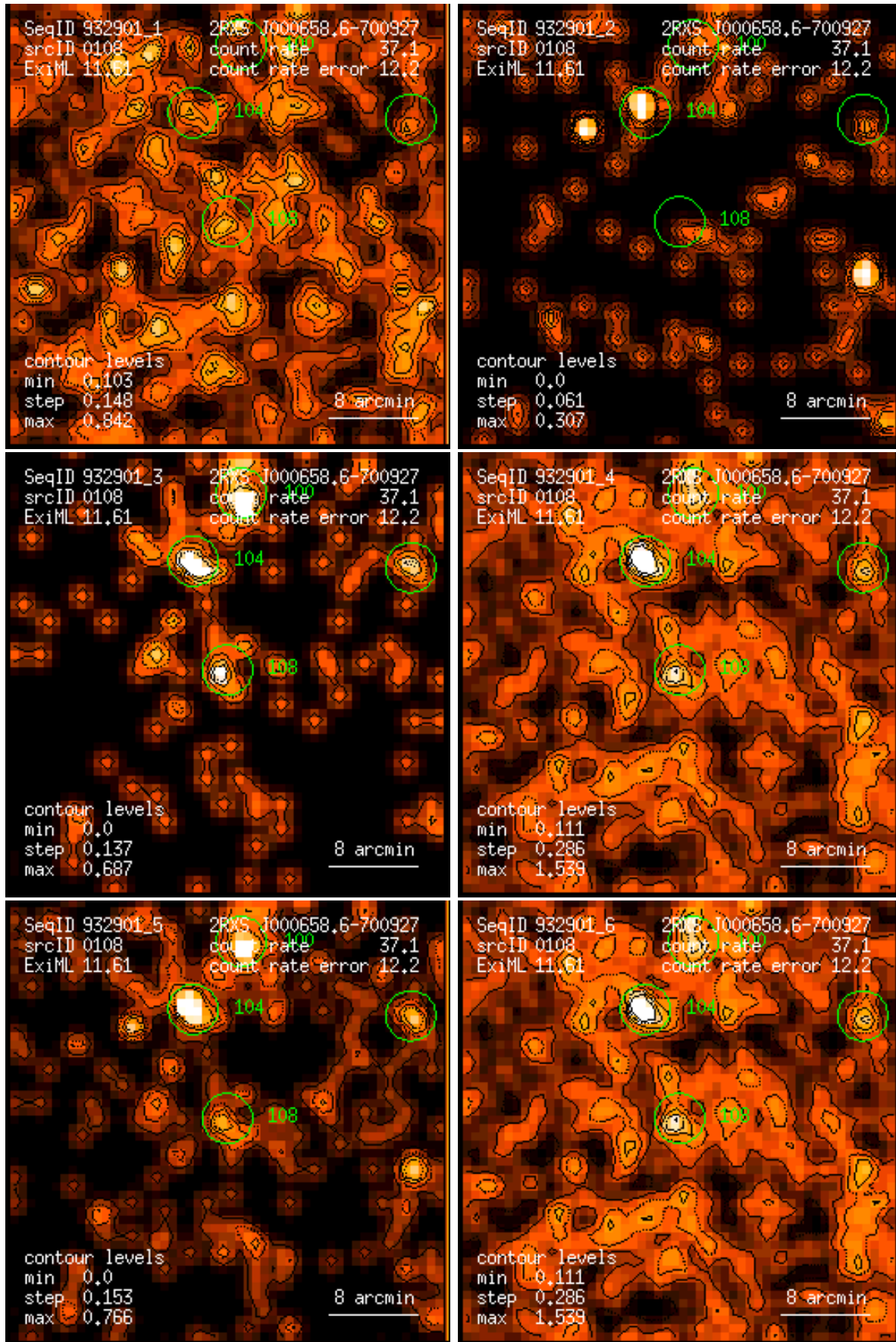
Figure 108: RASS 932901: detection 0108: band rate images, Gaussian filter: (1) PSPC channels 11 – 41, (2) 52 – 90, (3) 91 – 201, (4) 11 – 235, (5) 52 – 201, (6) 11 – 201. Broad band rates in counts/ks. Band rate contour levels in counts/ks/arcmin 2 .
