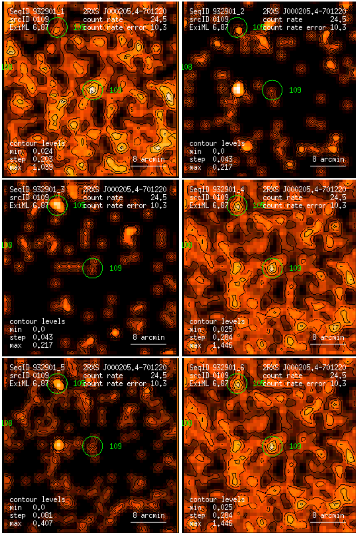
Figure 109: RASS 932901: detection 0109: band rate images, Gaussian filter: (1) PSPC channels 11 – 41, (2) 52 – 90, (3) 91 – 201, (4) 11 – 235, (5) 52 – 201, (6) 11 – 201. Broad band rates in counts/ks. Band rate contour levels in counts/ks/arcmin 2 .
