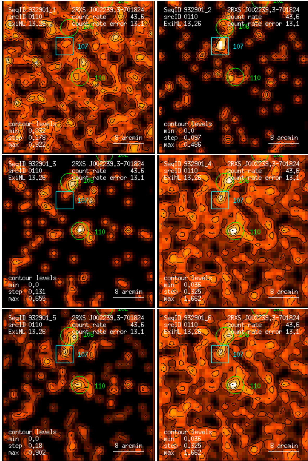
Figure 110: RASS 932901: detection 0110: band rate images, Gaussian filter: (1) PSPC channels 11 – 41, (2) 52 – 90, (3) 91 – 201, (4) 11 – 235, (5) 52 – 201, (6) 11 – 201. Broad band rates in counts/ks. Band rate contour levels in counts/ks/arcmin 2 .
