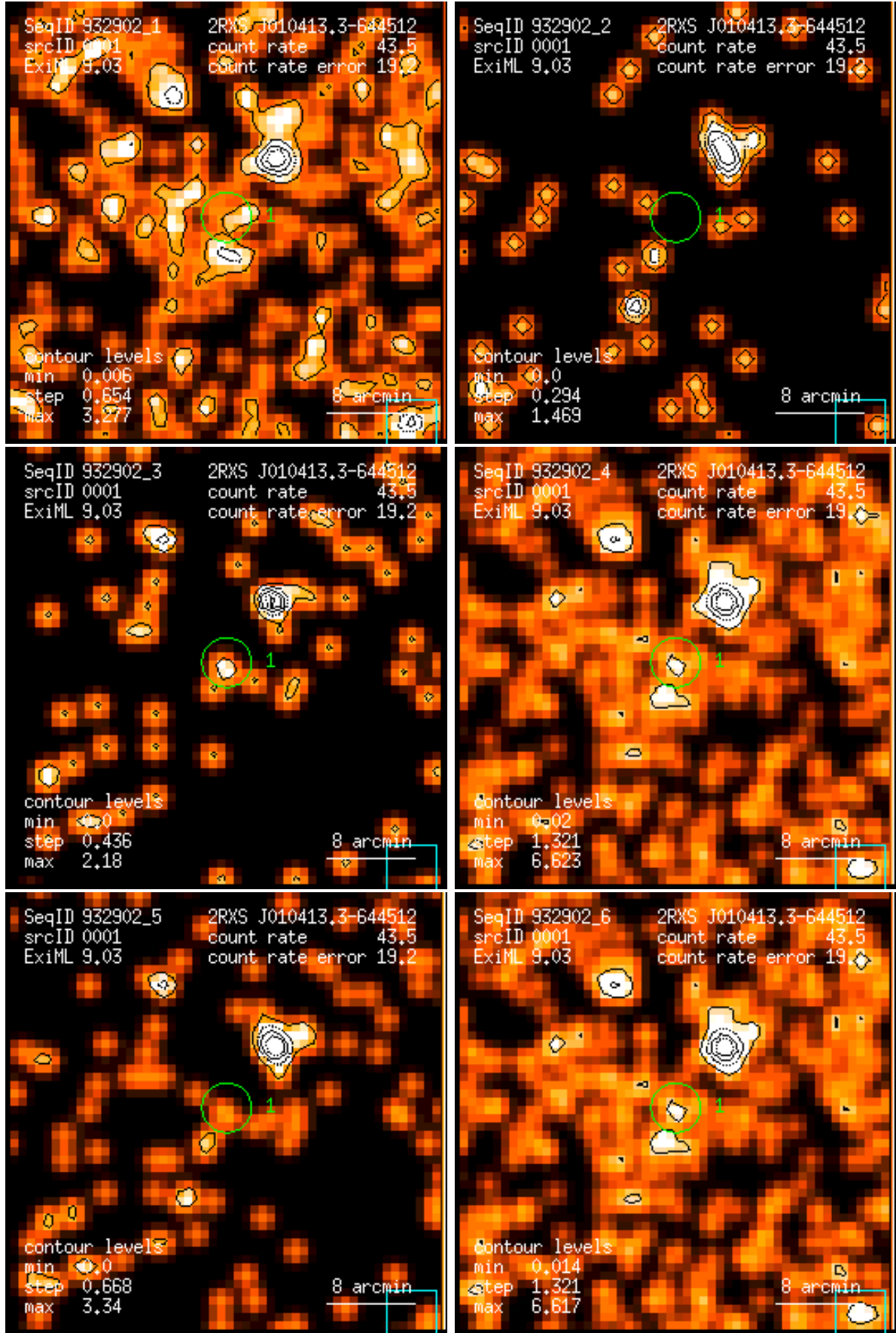
Figure 1: RASS 932902: detection 0001: band rate images, Gaussian filter: (1) PSPC channels 11 – 41, (2) 52 – 90, (3) 91 – 201, (4) 11 – 235, (5) 52 – 201, (6) 11 – 201. Broad band rates in counts/ks. Band rate contour levels in counts/ks/arcmin 2 .
