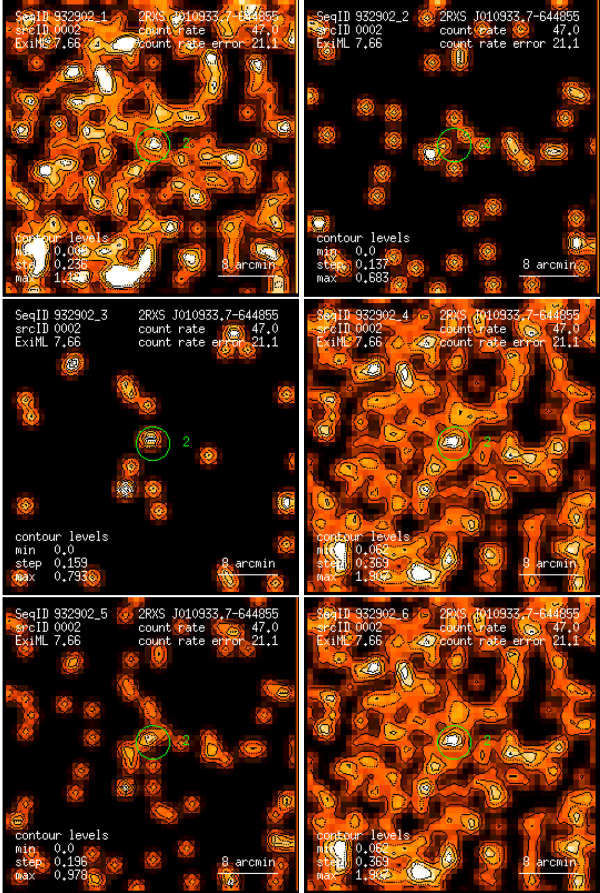
Figure 2: RASS 932902: detection 0002: band rate images, Gaussian filter: (1) PSPC channels 11 – 41, (2) 52 – 90, (3) 91 – 201, (4) 11 – 235, (5) 52 – 201, (6) 11 – 201. Broad band rates in counts/ks. Band rate contour levels in counts/ks/arcmin 2 .
