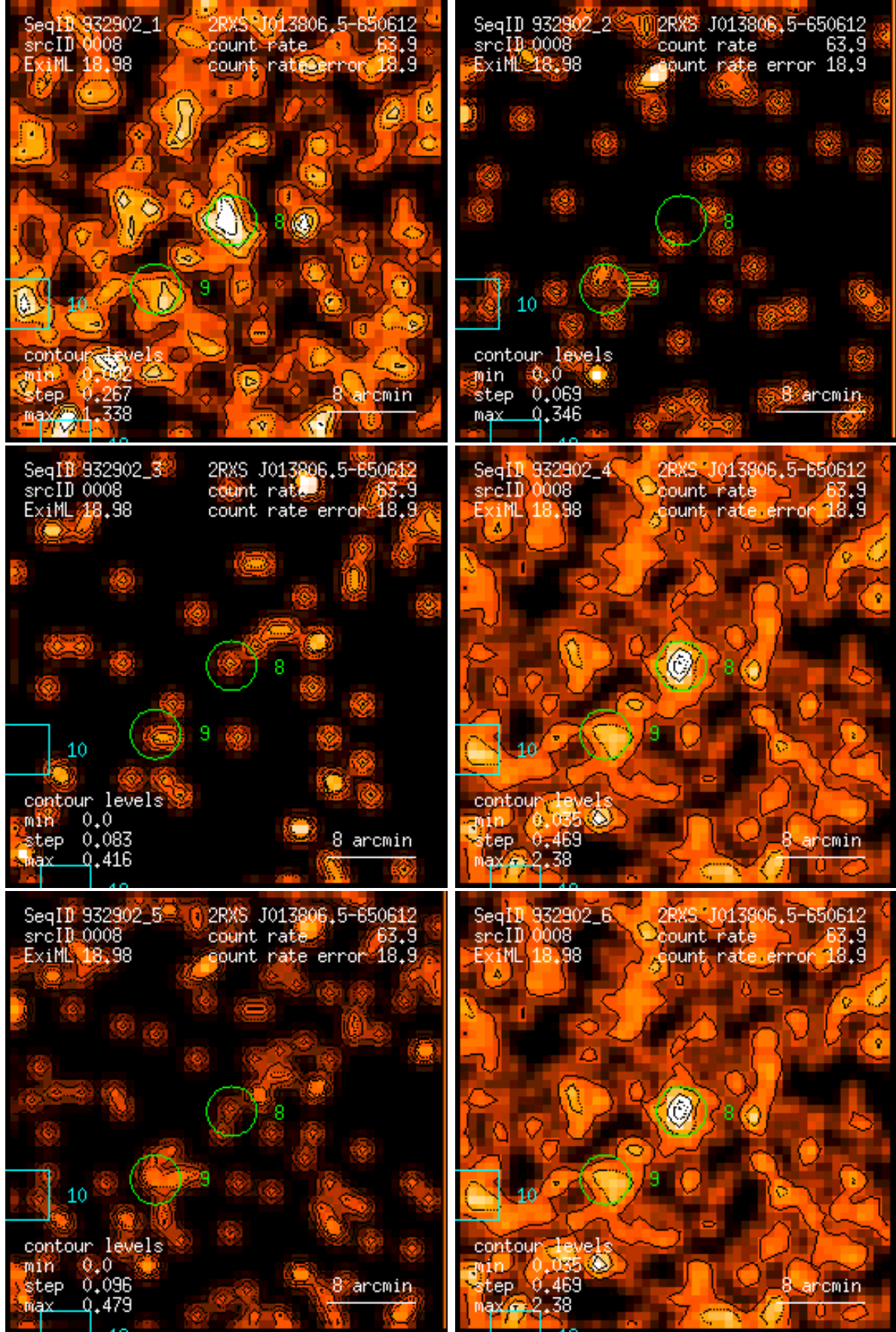
Figure 8: RASS 932902: detection 0008: band rate images, Gaussian filter: (1) PSPC channels 11 – 41, (2) 52 – 90, (3) 91 – 201, (4) 11 – 235, (5) 52 – 201, (6) 11 – 201. Broad band rates in counts/ks. Band rate contour levels in counts/ks/arcmin 2 .
