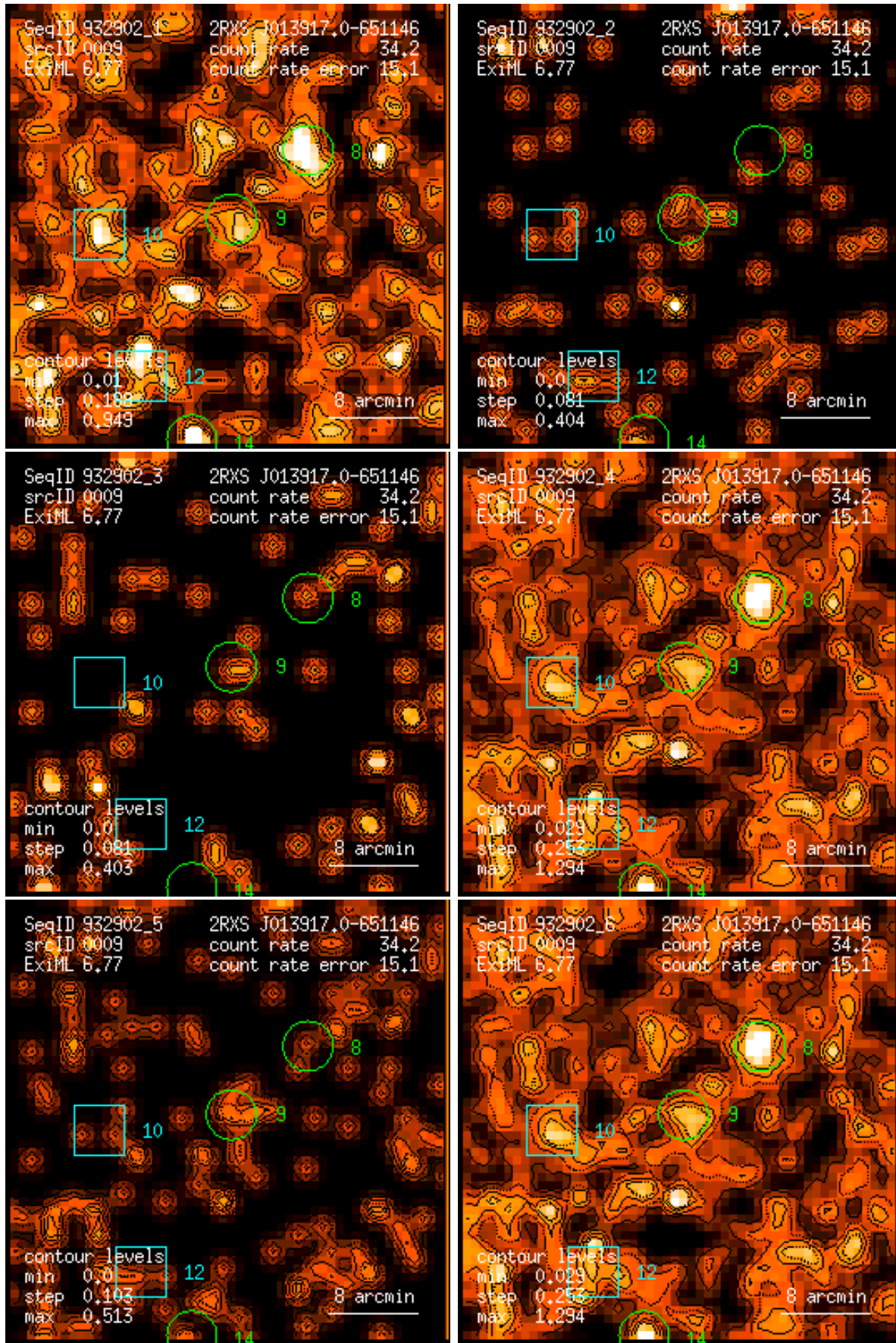
Figure 9: RASS 932902: detection 0009: band rate images, Gaussian filter: (1) PSPC channels 11 – 41, (2) 52 – 90, (3) 91 – 201, (4) 11 – 235, (5) 52 – 201, (6) 11 – 201. Broad band rates in counts/ks. Band rate contour levels in counts/ks/arcmin 2 .
