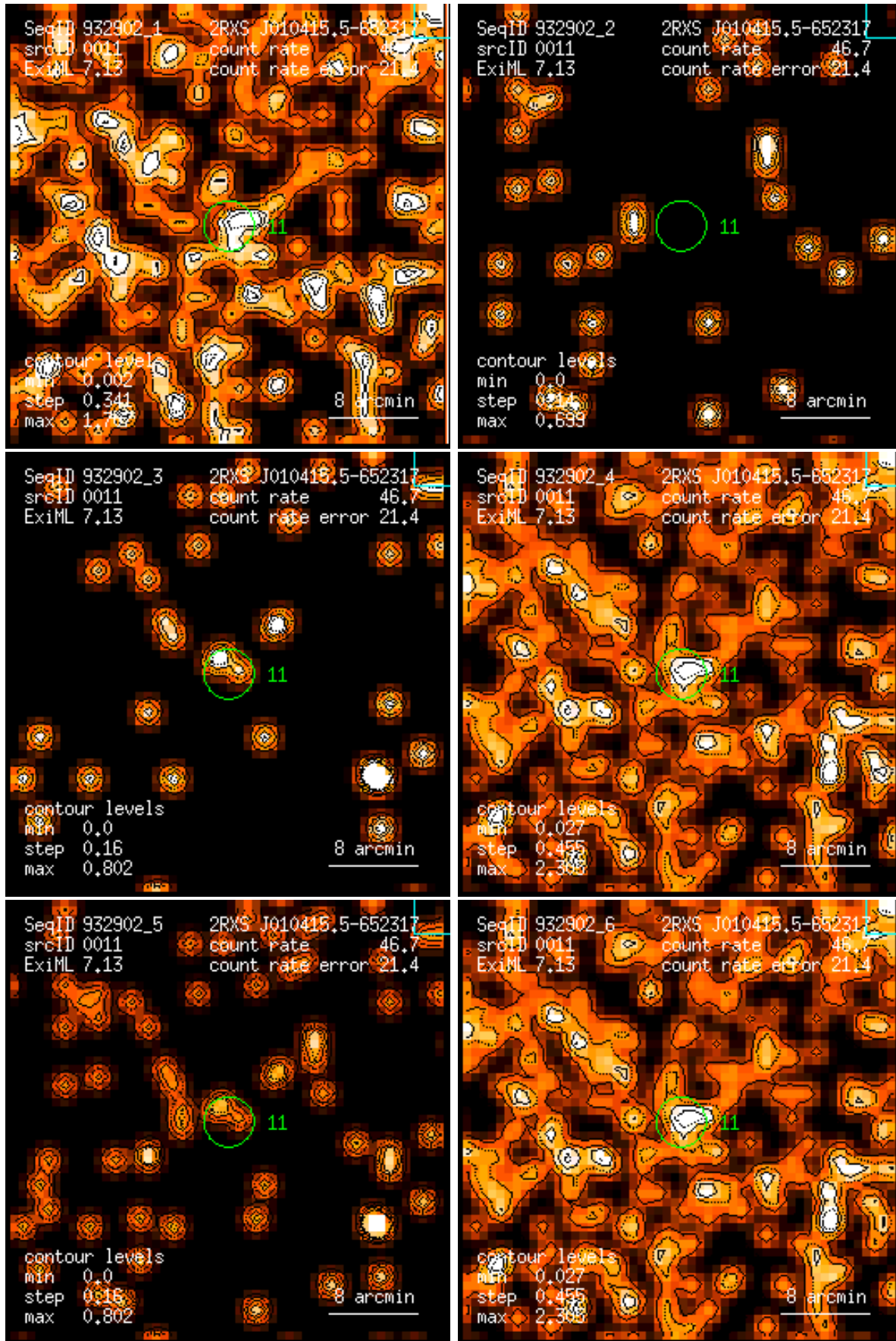
Figure 11: RASS 932902: detection 0011: band rate images, Gaussian filter: (1) PSPC channels 11 – 41, (2) 52 – 90, (3) 91 – 201, (4) 11 – 235, (5) 52 – 201, (6) 11 – 201. Broad band rates in counts/ks. Band rate contour levels in counts/ks/arcmin 2 .
