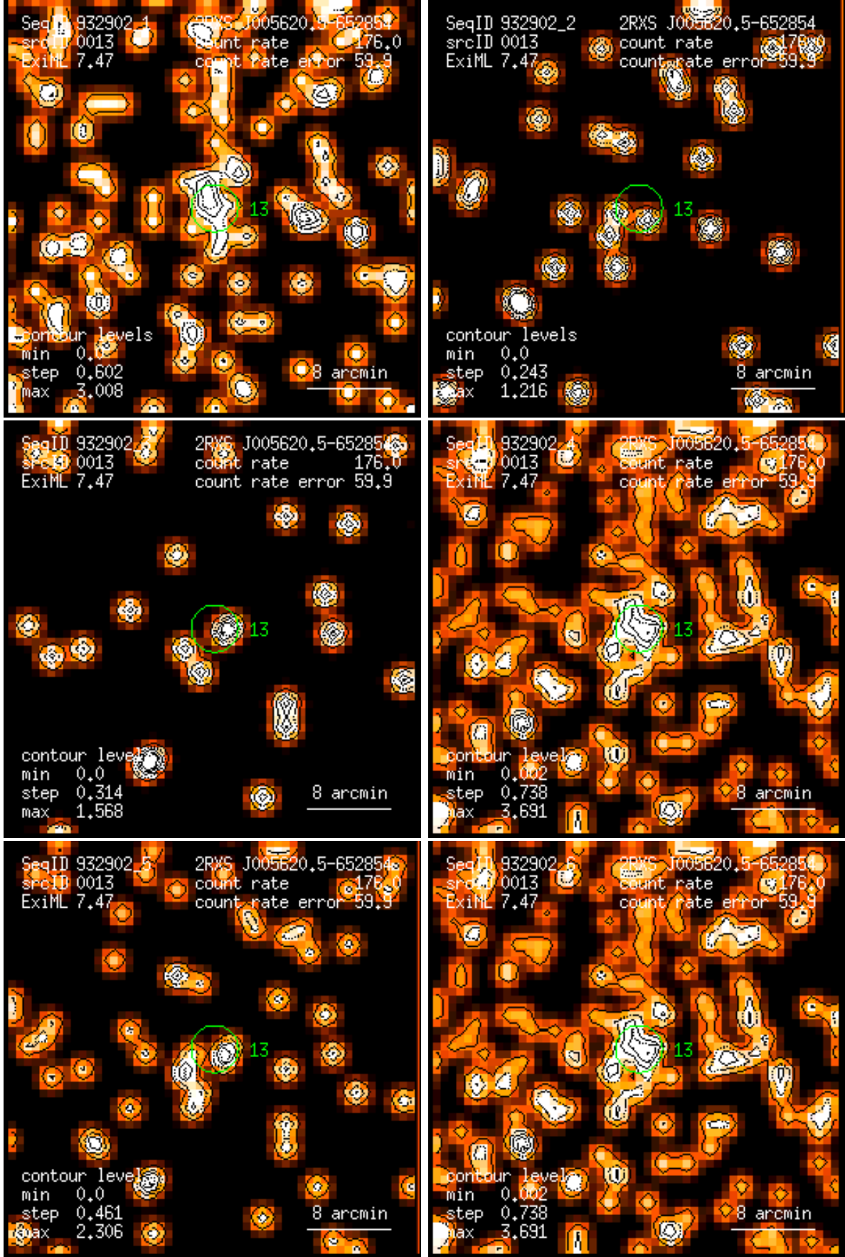
Figure 13: RASS 932902: detection 0013: band rate images, Gaussian filter: (1) PSPC channels 11 – 41, (2) 52 – 90, (3) 91 – 201, (4) 11 – 235, (5) 52 – 201, (6) 11 – 201. Broad band rates in counts/ks. Band rate contour levels in counts/ks/arcmin 2 .
