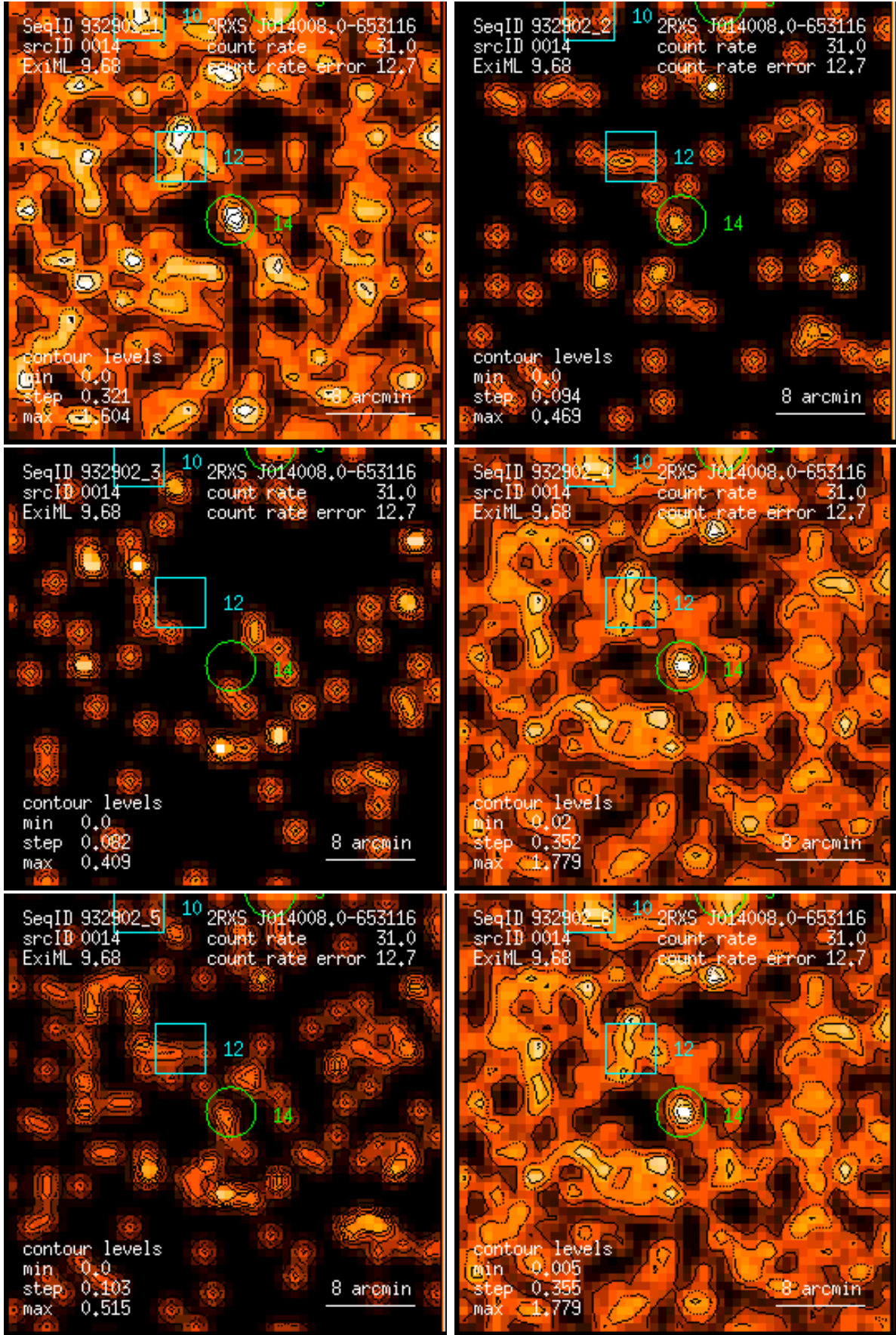
Figure 14: RASS 932902: detection 0014: band rate images, Gaussian filter: (1) PSPC channels 11 – 41, (2) 52 – 90, (3) 91 – 201, (4) 11 – 235, (5) 52 – 201, (6) 11 – 201. Broad band rates in counts/ks. Band rate contour levels in counts/ks/arcmin 2 .
