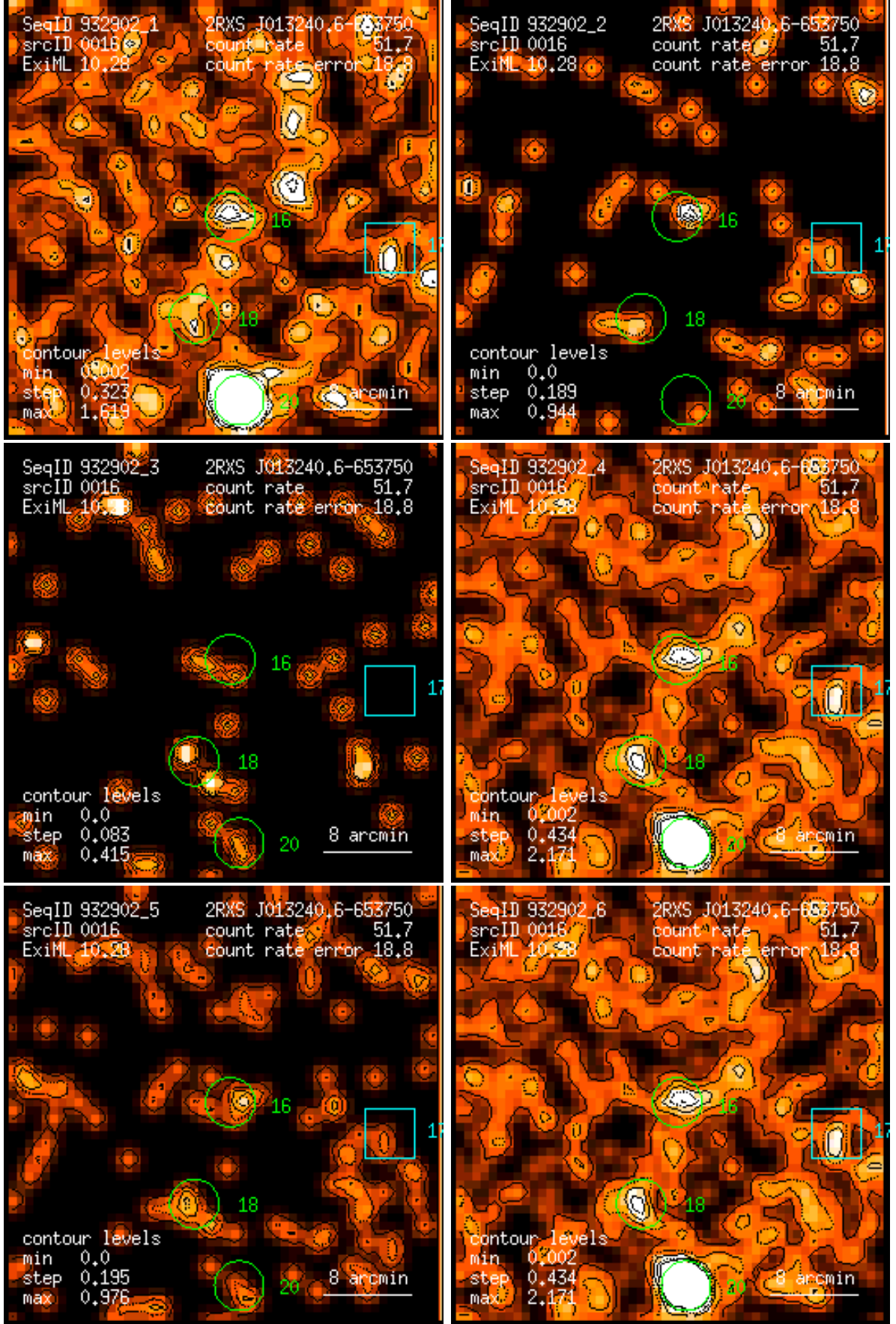
Figure 16: RASS 932902: detection 0016: band rate images, Gaussian filter: (1) PSPC channels 11 – 41, (2) 52 – 90, (3) 91 – 201, (4) 11 – 235, (5) 52 – 201, (6) 11 – 201. Broad band rates in counts/ks. Band rate contour levels in counts/ks/arcmin 2 .
