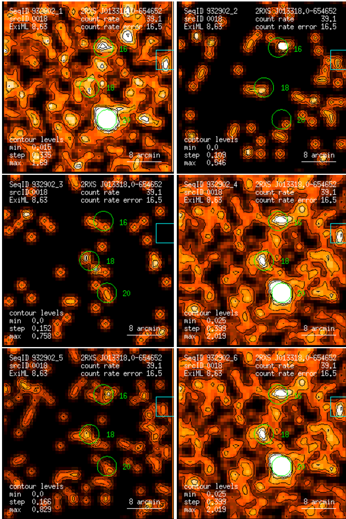
Figure 18: RASS 932902: detection 0018: band rate images, Gaussian filter: (1) PSPC channels 11 – 41, (2) 52 – 90, (3) 91 – 201, (4) 11 – 235, (5) 52 – 201, (6) 11 – 201. Broad band rates in counts/ks. Band rate contour levels in counts/ks/arcmin 2 .
