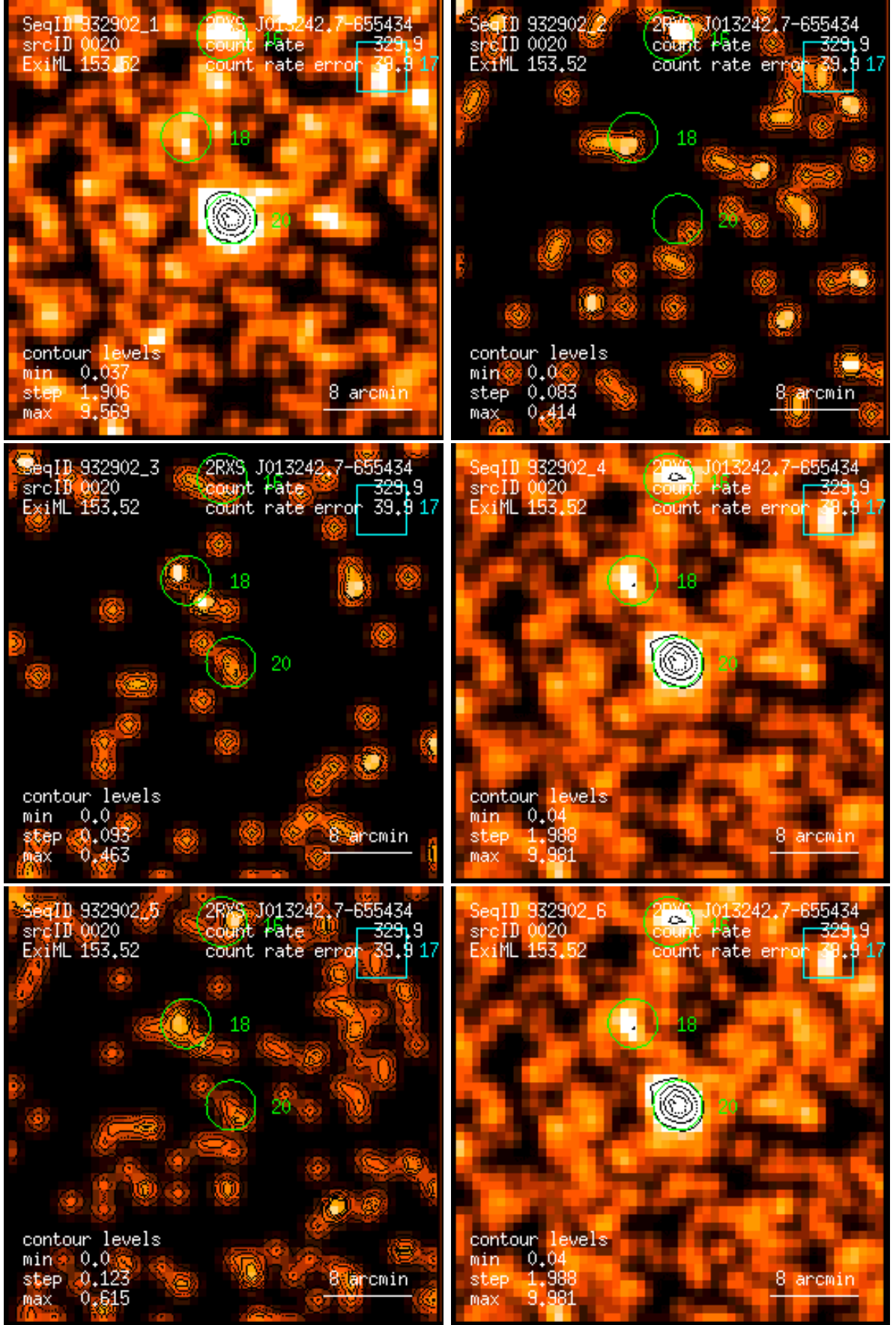
Figure 20: RASS 932902: detection 0020: band rate images, Gaussian filter: (1) PSPC channels 11 – 41, (2) 52 – 90, (3) 91 – 201, (4) 11 – 235, (5) 52 – 201, (6) 11 – 201. Broad band rates in counts/ks. Band rate contour levels in counts/ks/arcmin 2 .
