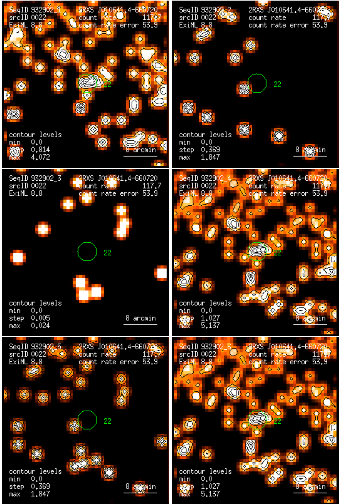
Figure 22: RASS 932902: detection 0022: band rate images, Gaussian filter: (1) PSPC channels 11 – 41, (2) 52 – 90, (3) 91 – 201, (4) 11 – 235, (5) 52 – 201, (6) 11 – 201. Broad band rates in counts/ks. Band rate contour levels in counts/ks/arcmin 2 .
