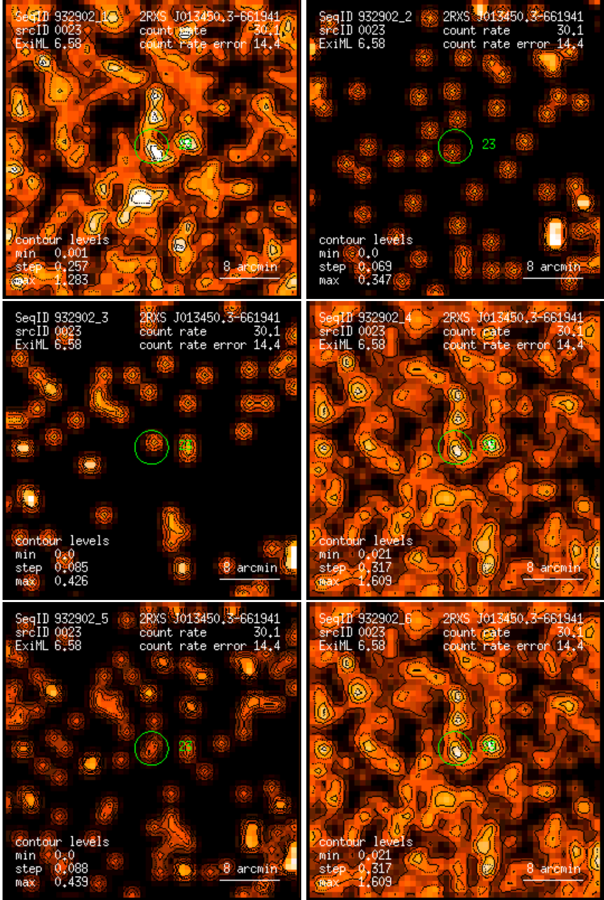
Figure 23: RASS 932902: detection 0023: band rate images, Gaussian filter: (1) PSPC channels 11 – 41, (2) 52 – 90, (3) 91 – 201, (4) 11 – 235, (5) 52 – 201, (6) 11 – 201. Broad band rates in counts/ks. Band rate contour levels in counts/ks/arcmin 2 .
