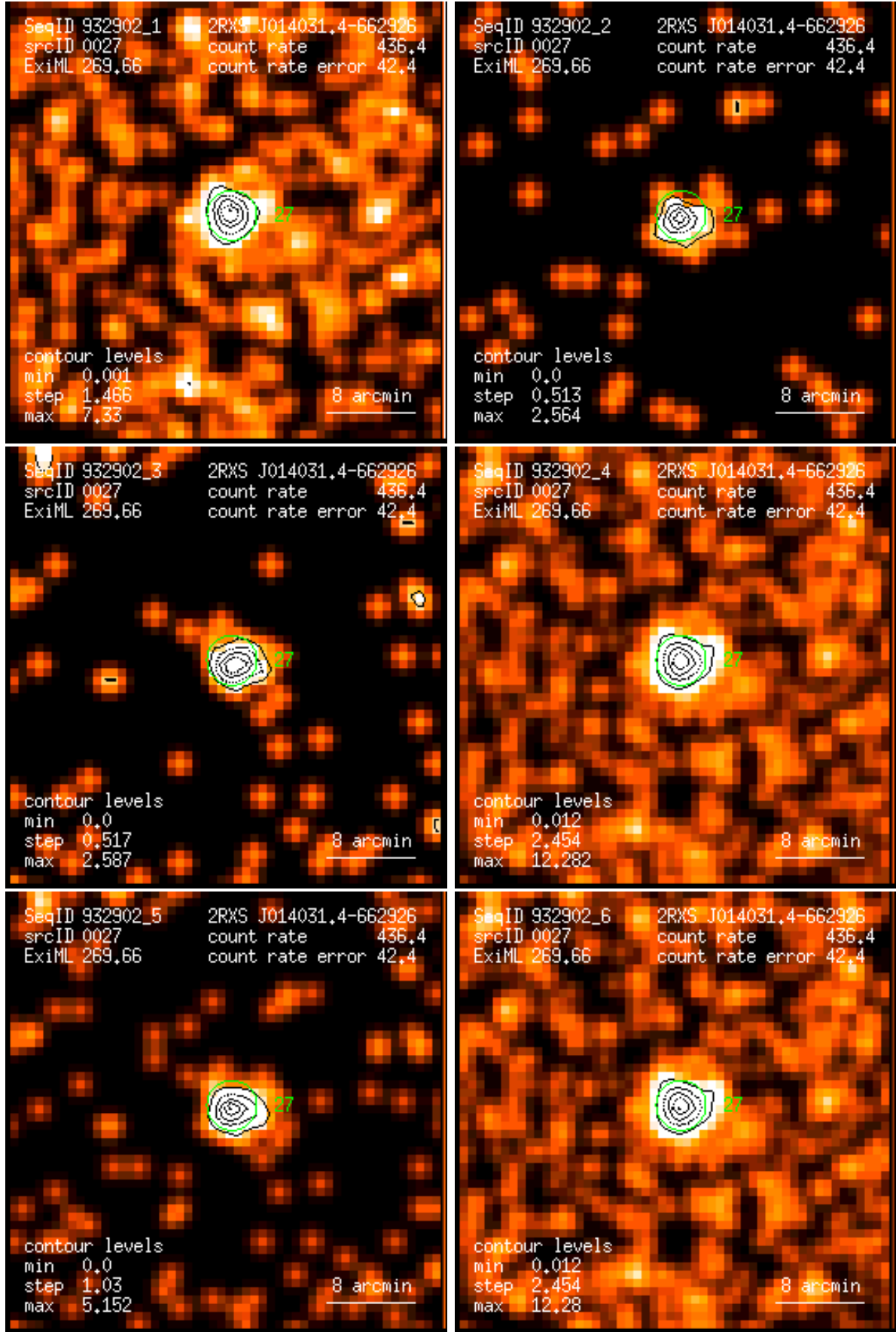
Figure 27: RASS 932902: detection 0027: band rate images, Gaussian filter: (1) PSPC channels 11 – 41, (2) 52 – 90, (3) 91 – 201, (4) 11 – 235, (5) 52 – 201, (6) 11 – 201. Broad band rates in counts/ks. Band rate contour levels in counts/ks/arcmin 2 .
