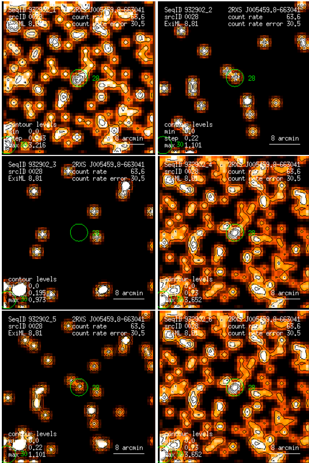
Figure 28: RASS 932902: detection 0028: band rate images, Gaussian filter: (1) PSPC channels 11 – 41, (2) 52 – 90, (3) 91 – 201, (4) 11 – 235, (5) 52 – 201, (6) 11 – 201. Broad band rates in counts/ks. Band rate contour levels in counts/ks/arcmin 2 .
