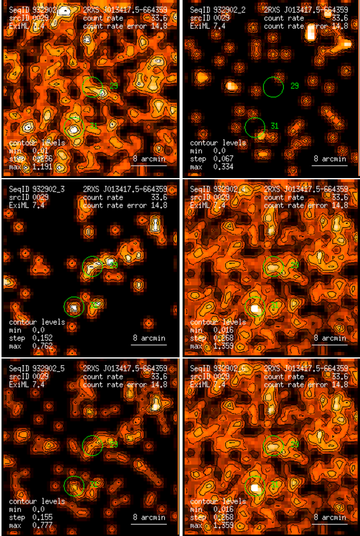
Figure 29: RASS 932902: detection 0029: band rate images, Gaussian filter: (1) PSPC channels 11 – 41, (2) 52 – 90, (3) 91 – 201, (4) 11 – 235, (5) 52 – 201, (6) 11 – 201. Broad band rates in counts/ks. Band rate contour levels in counts/ks/arcmin 2 .
