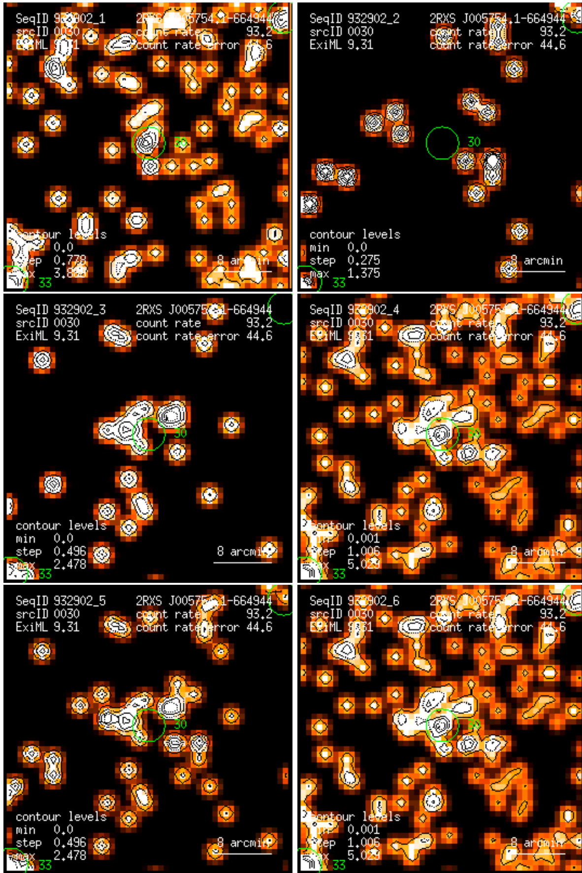
Figure 30: RASS 932902: detection 0030: band rate images, Gaussian filter: (1) PSPC channels 11 – 41, (2) 52 – 90, (3) 91 – 201, (4) 11 – 235, (5) 52 – 201, (6) 11 – 201. Broad band rates in counts/ks. Band rate contour levels in counts/ks/arcmin 2 .
