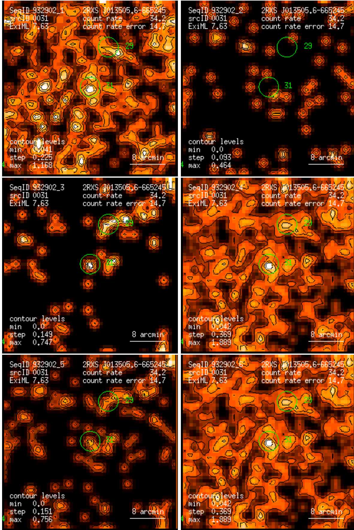
Figure 31: RASS 932902: detection 0031: band rate images, Gaussian filter: (1) PSPC channels 11 – 41, (2) 52 – 90, (3) 91 – 201, (4) 11 – 235, (5) 52 – 201, (6) 11 – 201. Broad band rates in counts/ks. Band rate contour levels in counts/ks/arcmin 2 .
