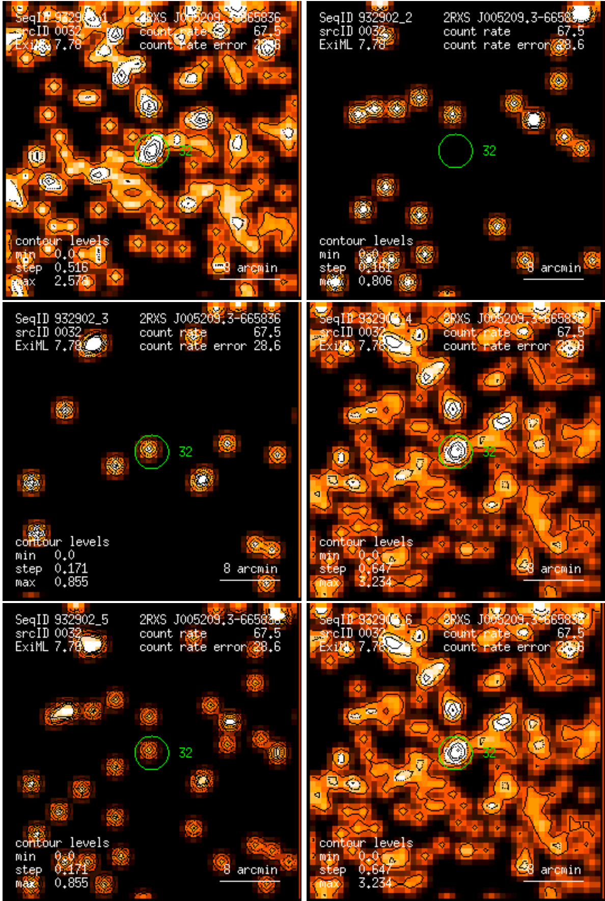
Figure 32: RASS 932902: detection 0032: band rate images, Gaussian filter: (1) PSPC channels 11 – 41, (2) 52 – 90, (3) 91 – 201, (4) 11 – 235, (5) 52 – 201, (6) 11 – 201. Broad band rates in counts/ks. Band rate contour levels in counts/ks/arcmin 2 .
