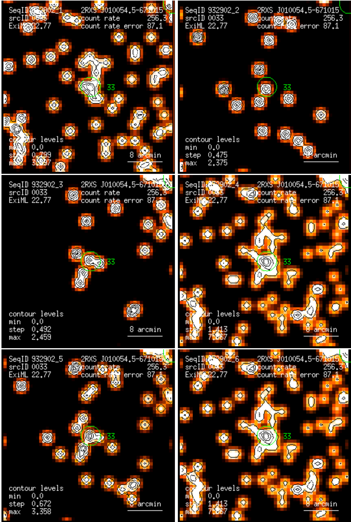
Figure 33: RASS 932902: detection 0033: band rate images, Gaussian filter: (1) PSPC channels 11 – 41, (2) 52 – 90, (3) 91 – 201, (4) 11 – 235, (5) 52 – 201, (6) 11 – 201. Broad band rates in counts/ks. Band rate contour levels in counts/ks/arcmin 2 .
