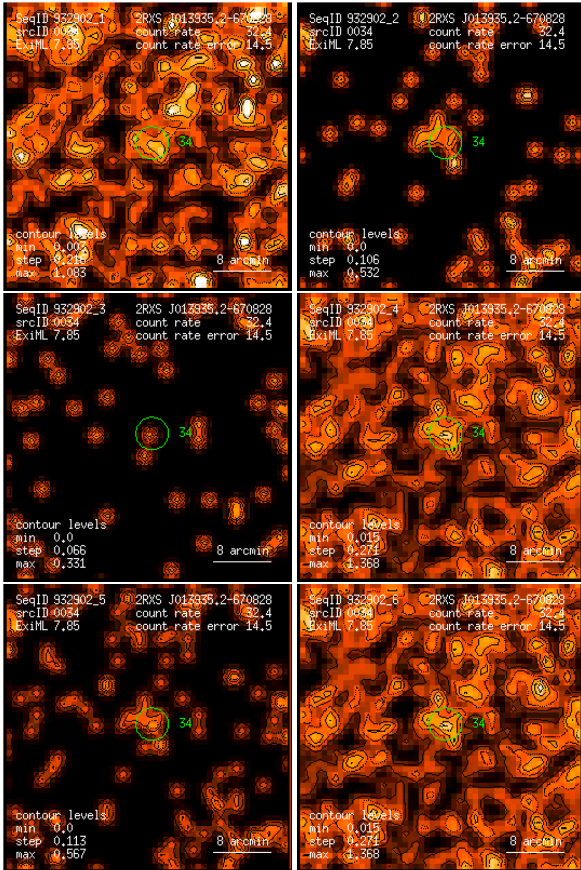
Figure 34: RASS 932902: detection 0034: band rate images, Gaussian filter: (1) PSPC channels 11 – 41, (2) 52 – 90, (3) 91 – 201, (4) 11 – 235, (5) 52 – 201, (6) 11 – 201. Broad band rates in counts/ks. Band rate contour levels in counts/ks/arcmin 2 .
