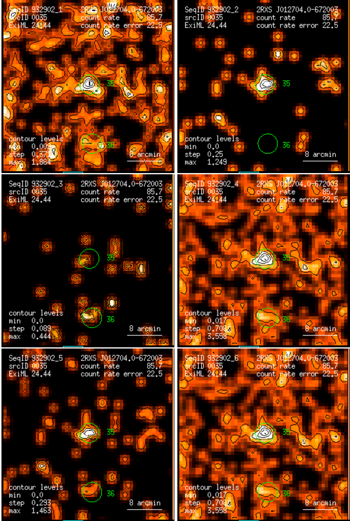
Figure 35: RASS 932902: detection 0035: band rate images, Gaussian filter: (1) PSPC channels 11 – 41, (2) 52 – 90, (3) 91 – 201, (4) 11 – 235, (5) 52 – 201, (6) 11 – 201. Broad band rates in counts/ks. Band rate contour levels in counts/ks/arcmin 2 .
