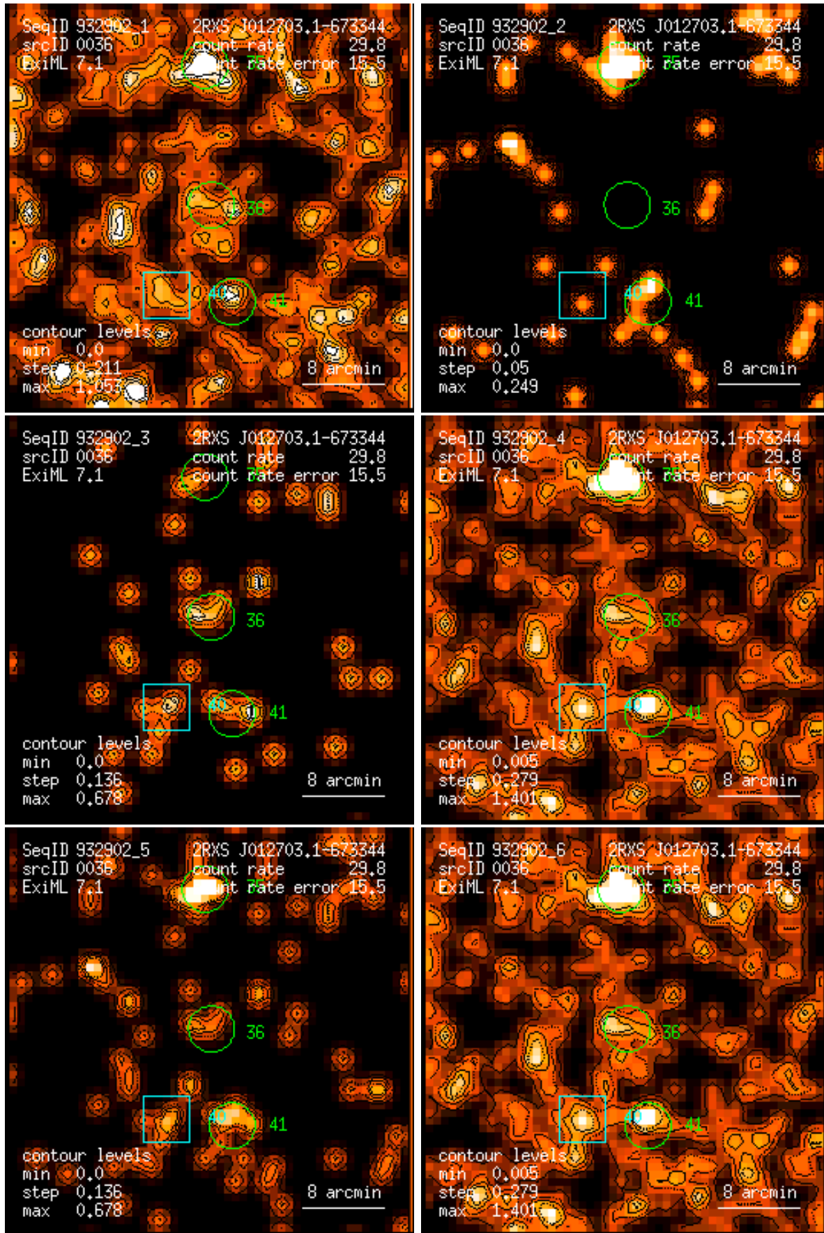
Figure 36: RASS 932902: detection 0036: band rate images, Gaussian filter: (1) PSPC channels 11 – 41, (2) 52 – 90, (3) 91 – 201, (4) 11 – 235, (5) 52 – 201, (6) 11 – 201. Broad band rates in counts/ks. Band rate contour levels in counts/ks/arcmin 2 .
