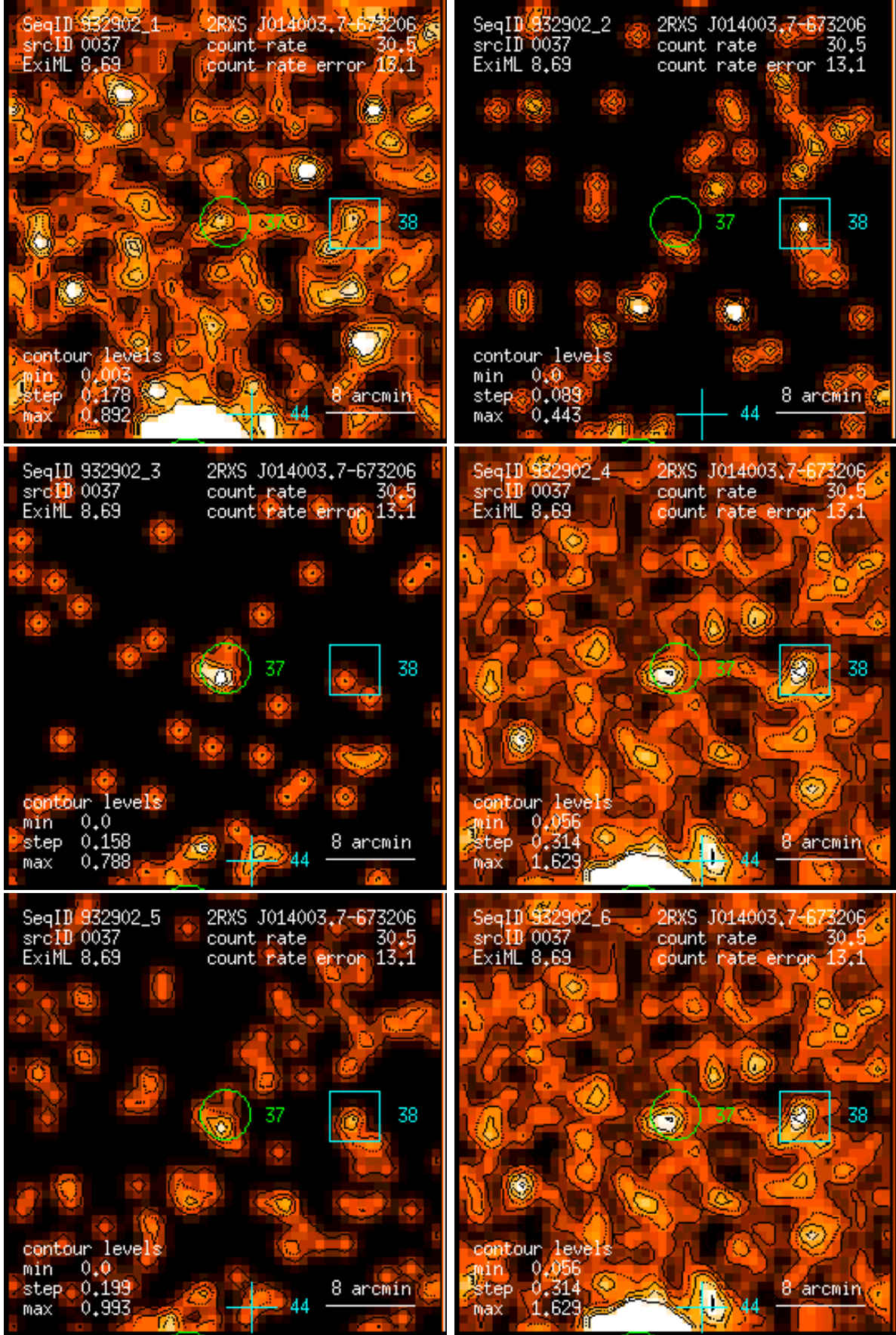
Figure 37: RASS 932902: detection 0037: band rate images, Gaussian filter: (1) PSPC channels 11 – 41, (2) 52 – 90, (3) 91 – 201, (4) 11 – 235, (5) 52 – 201, (6) 11 – 201. Broad band rates in counts/ks. Band rate contour levels in counts/ks/arcmin 2 .
