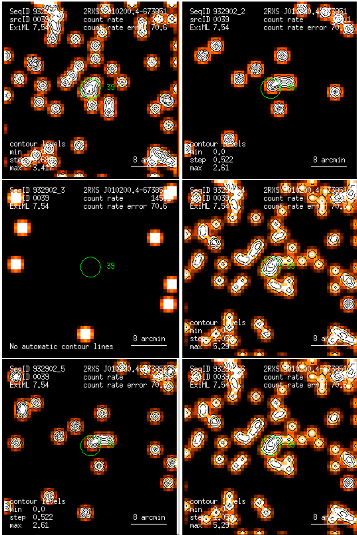
Figure 39: RASS 932902: detection 0039: band rate images, Gaussian filter: (1) PSPC channels 11 – 41, (2) 52 – 90, (3) 91 – 201, (4) 11 – 235, (5) 52 – 201, (6) 11 – 201. Broad band rates in counts/ks. Band rate contour levels in counts/ks/arcmin 2 .
