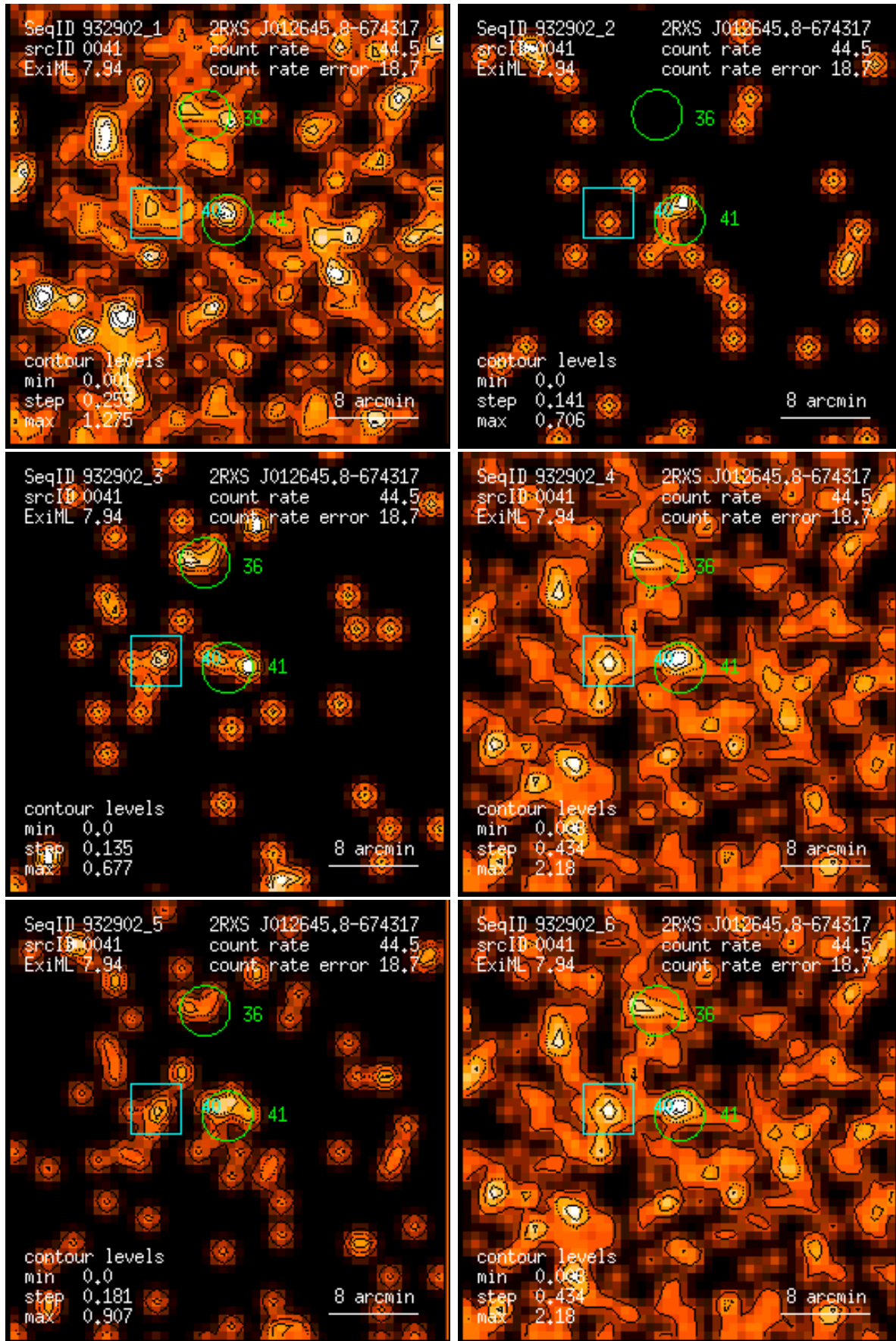
Figure 41: RASS 932902: detection 0041: band rate images, Gaussian filter: (1) PSPC channels 11 – 41, (2) 52 – 90, (3) 91 – 201, (4) 11 – 235, (5) 52 – 201, (6) 11 – 201. Broad band rates in counts/ks. Band rate contour levels in counts/ks/arcmin 2 .
