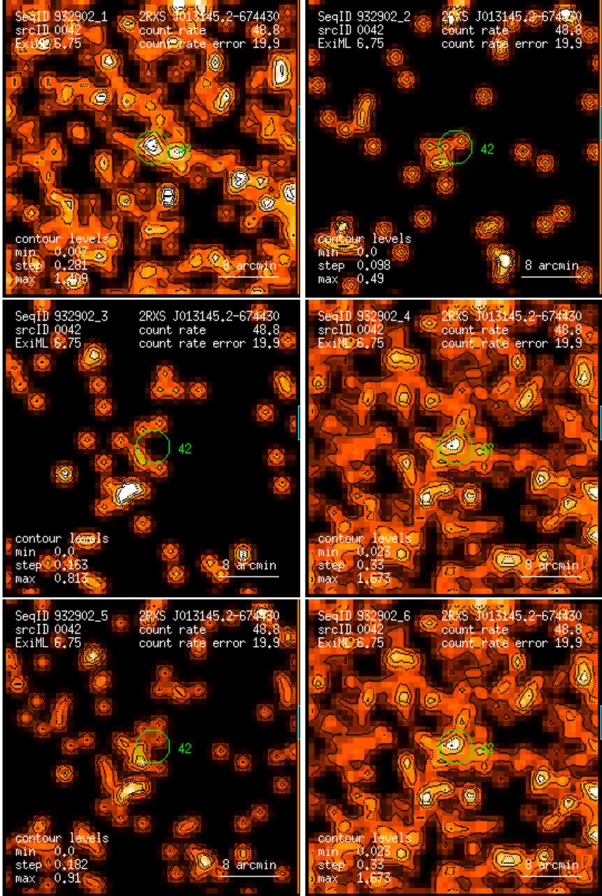
Figure 42: RASS 932902: detection 0042: band rate images, Gaussian filter: (1) PSPC channels 11 – 41, (2) 52 – 90, (3) 91 – 201, (4) 11 – 235, (5) 52 – 201, (6) 11 – 201. Broad band rates in counts/ks. Band rate contour levels in counts/ks/arcmin 2 .
