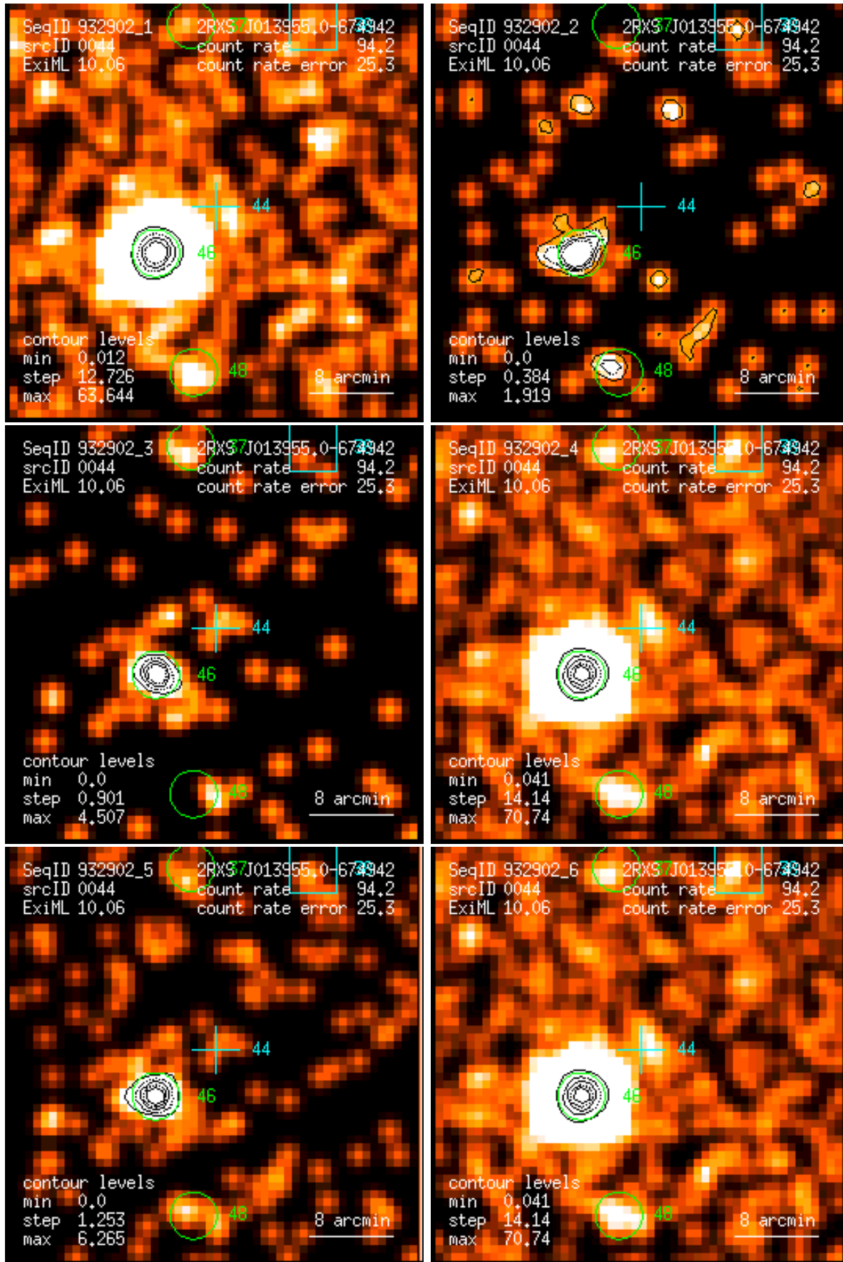
Figure 44: RASS 932902: detection 0044: band rate images, Gaussian filter: (1) PSPC channels 11 – 41, (2) 52 – 90, (3) 91 – 201, (4) 11 – 235, (5) 52 – 201, (6) 11 – 201. Broad band rates in counts/ks. Band rate contour levels in counts/ks/arcmin 2 .
