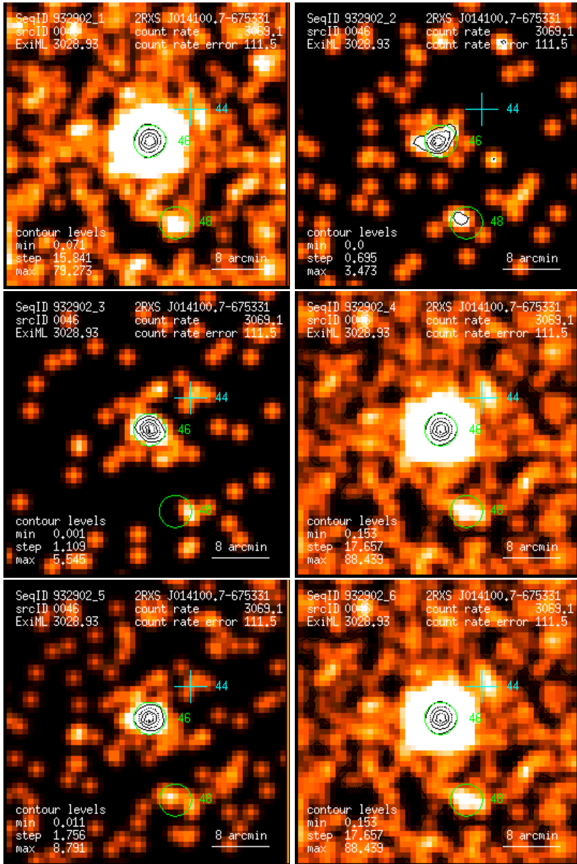
Figure 46: RASS 932902: detection 0046: band rate images, Gaussian filter: (1) PSPC channels 11 – 41, (2) 52 – 90, (3) 91 – 201, (4) 11 – 235, (5) 52 – 201, (6) 11 – 201. Broad band rates in counts/ks. Band rate contour levels in counts/ks/arcmin 2 .
