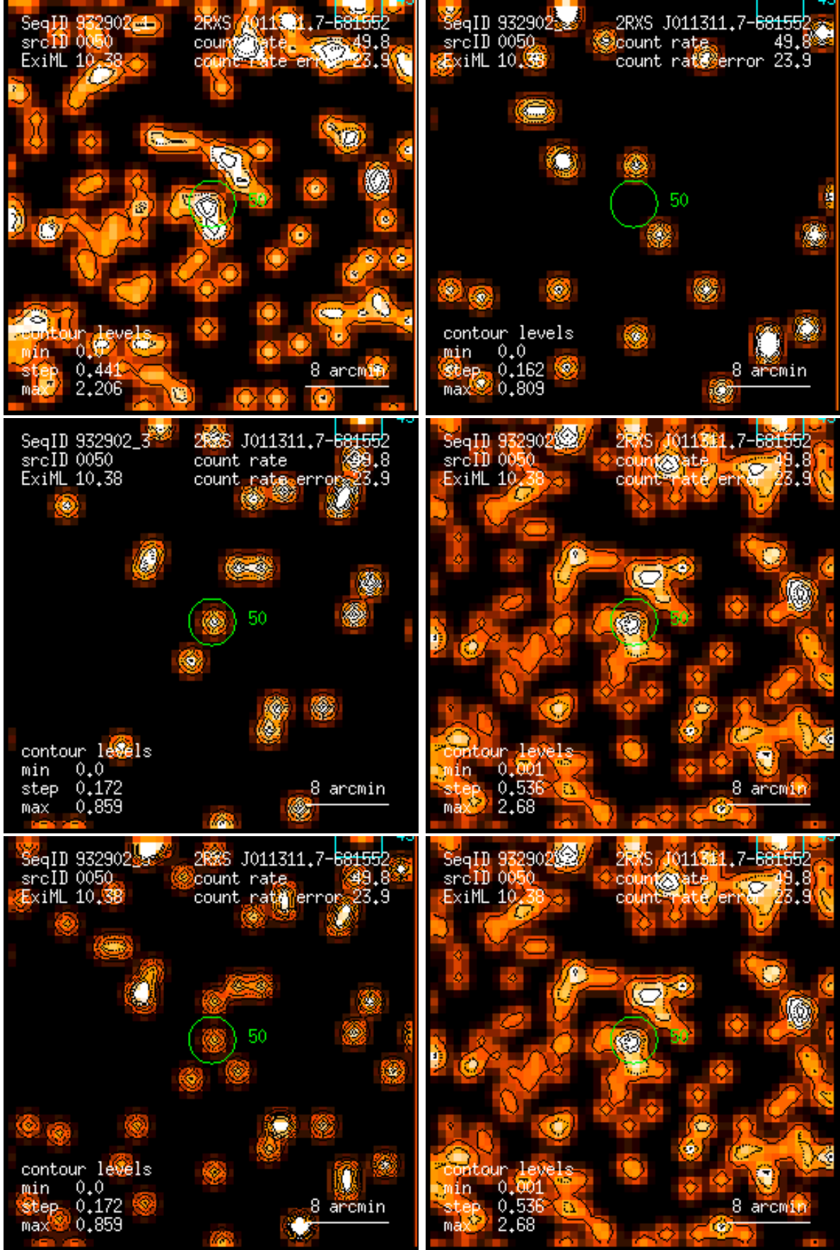
Figure 50: RASS 932902: detection 0050: band rate images, Gaussian filter: (1) PSPC channels 11 – 41, (2) 52 – 90, (3) 91 – 201, (4) 11 – 235, (5) 52 – 201, (6) 11 – 201. Broad band rates in counts/ks. Band rate contour levels in counts/ks/arcmin 2 .
