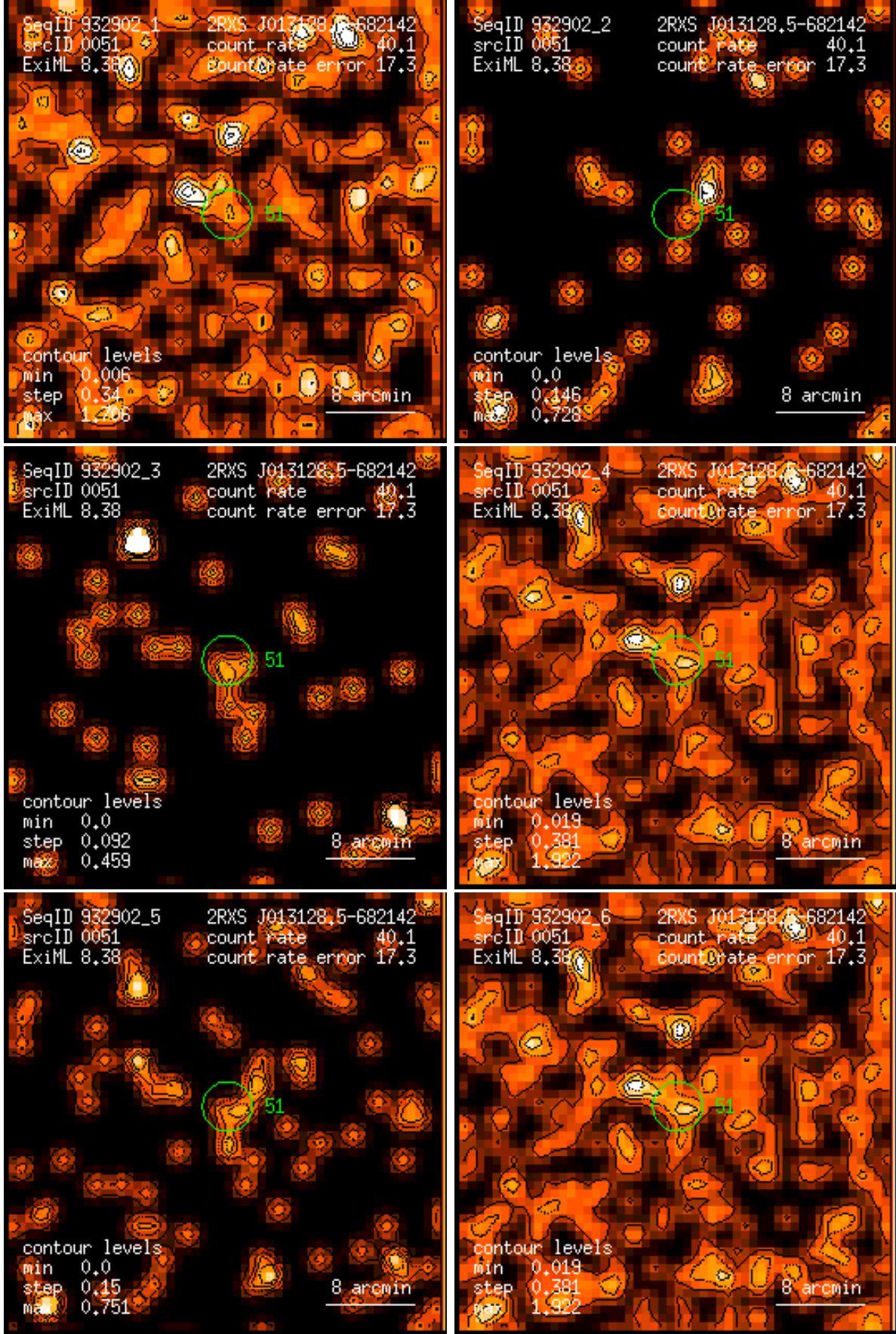
Figure 51: RASS 932902: detection 0051: band rate images, Gaussian filter: (1) PSPC channels 11 – 41, (2) 52 – 90, (3) 91 – 201, (4) 11 – 235, (5) 52 – 201, (6) 11 – 201. Broad band rates in counts/ks. Band rate contour levels in counts/ks/arcmin 2 .
