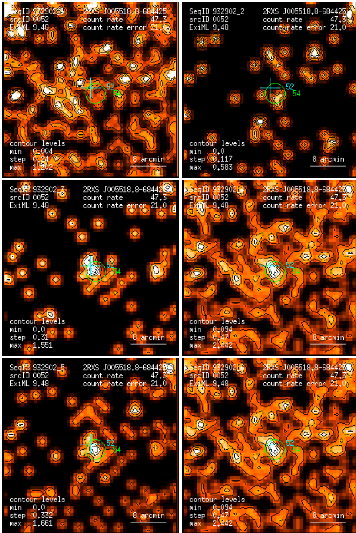
Figure 52: RASS 932902: detection 0052: band rate images, Gaussian filter: (1) PSPC channels 11 – 41, (2) 52 – 90, (3) 91 – 201, (4) 11 – 235, (5) 52 – 201, (6) 11 – 201. Broad band rates in counts/ks. Band rate contour levels in counts/ks/arcmin 2 .
